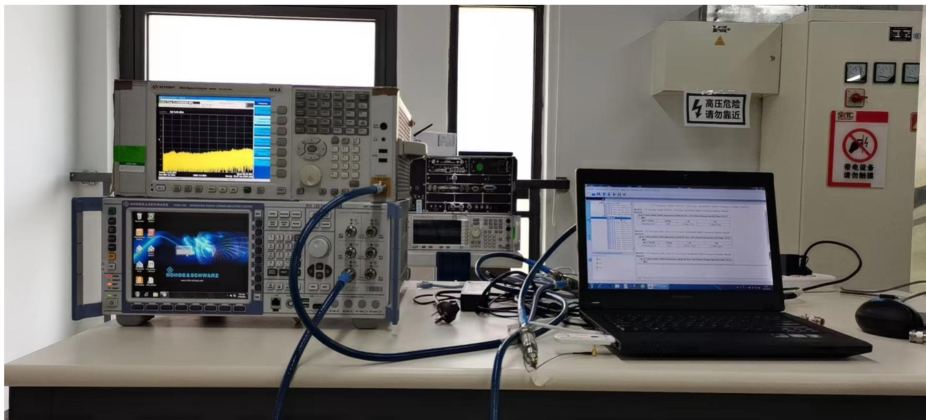
'RF Conducted Test setup (GSM/WCDMA/LTE)
