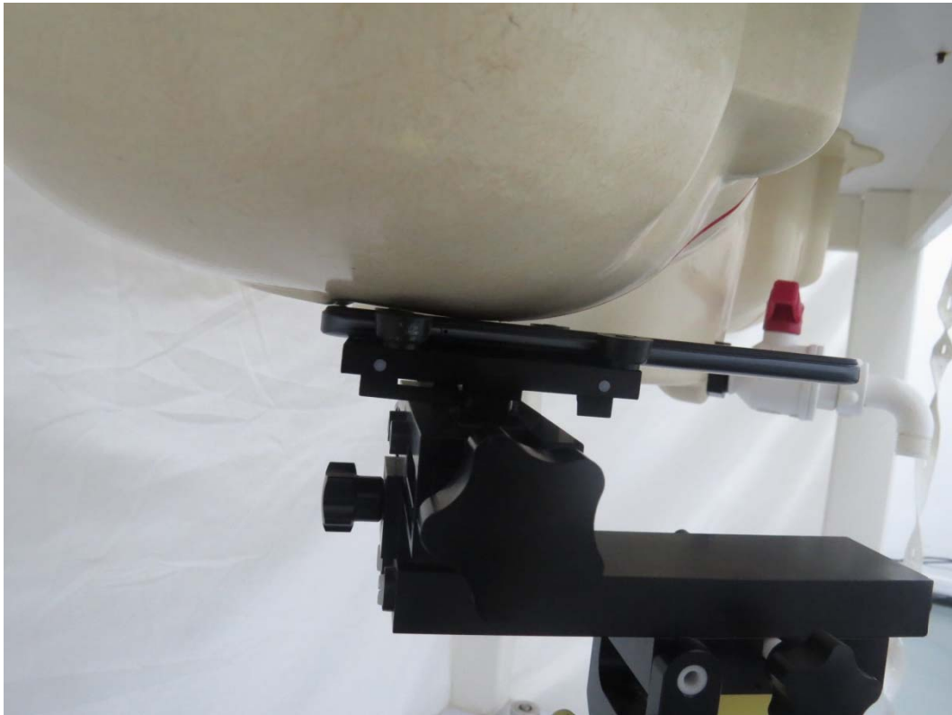
Picture 3: Right Hand Touch Cheek Position
