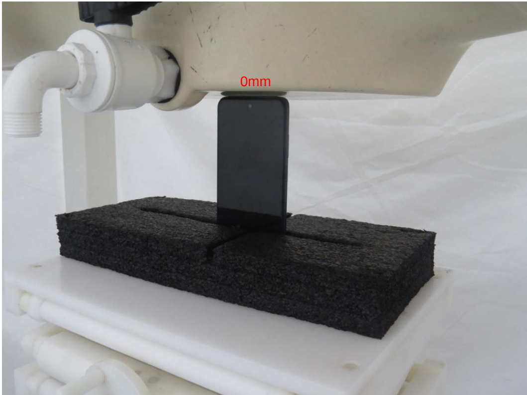
Picture 17: Top Side, the distance from handset to the bottom of the Phantom is 0mm
