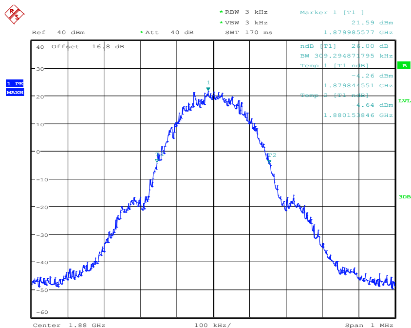
Figure 15: 26dB & 99% Occupied Bandwidth, GPRS1900, Mode B
