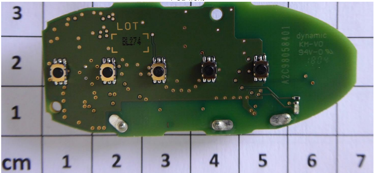
PCB front
