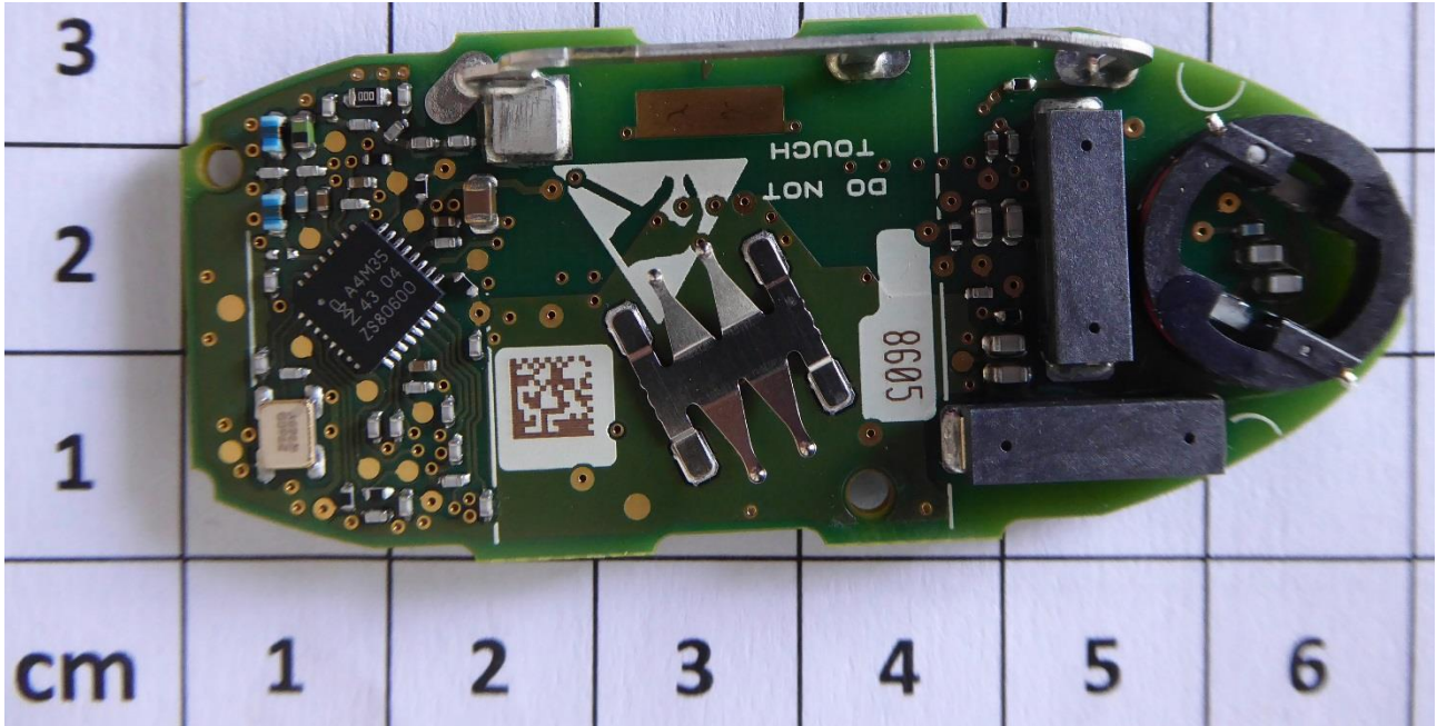
PCB front
