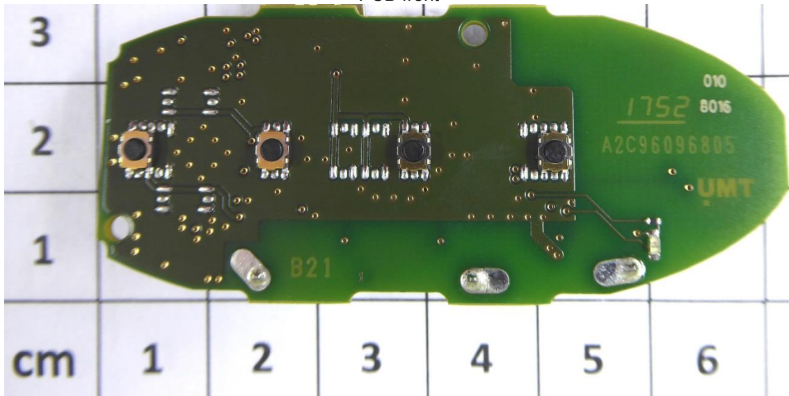
PCB front
