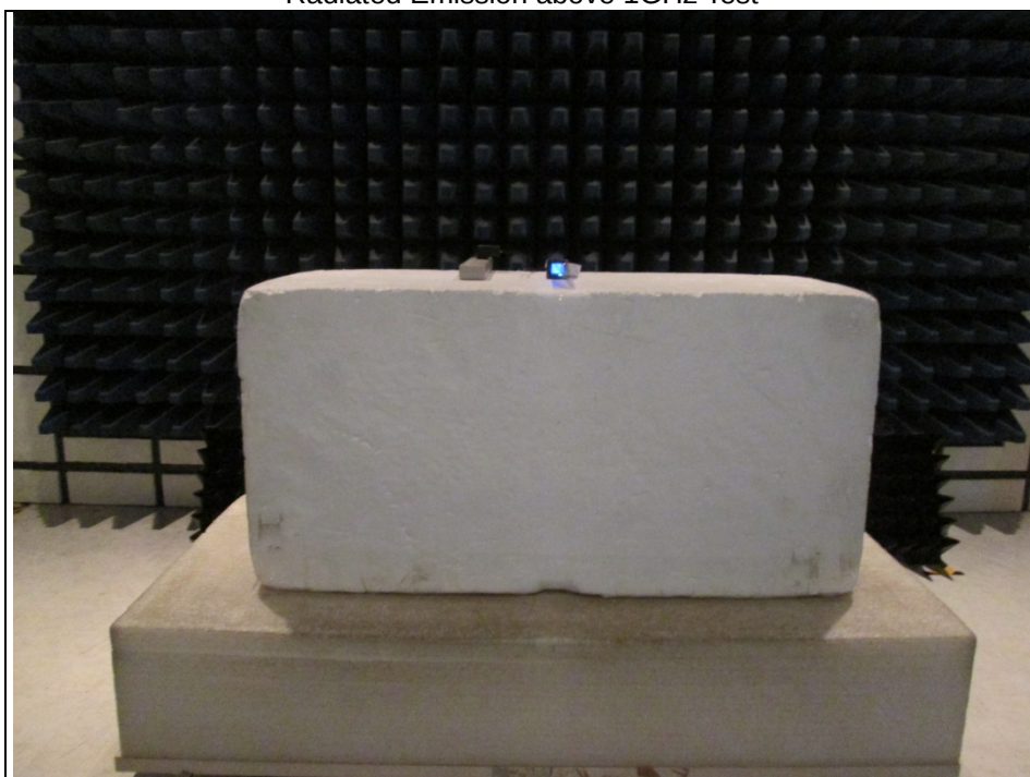
Radiated Emission above 1GHz Test
