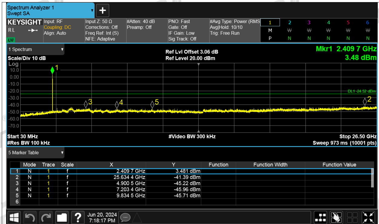
Tx. Spurious NVNT be20 52+26RU Index 38+4 2412MHz Ant2 Ref
