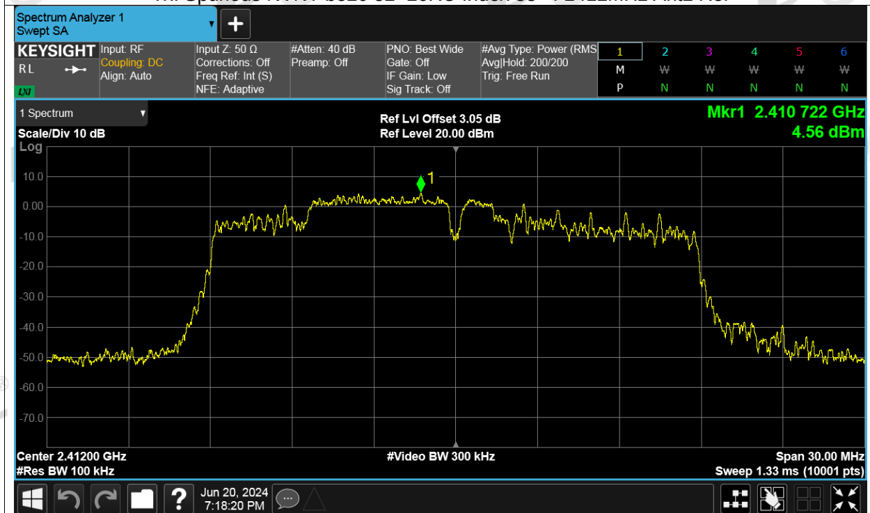
Tx. Spurious NVNT be20 52+26RU Index 38+4 2412MHz Ant2 Emission
