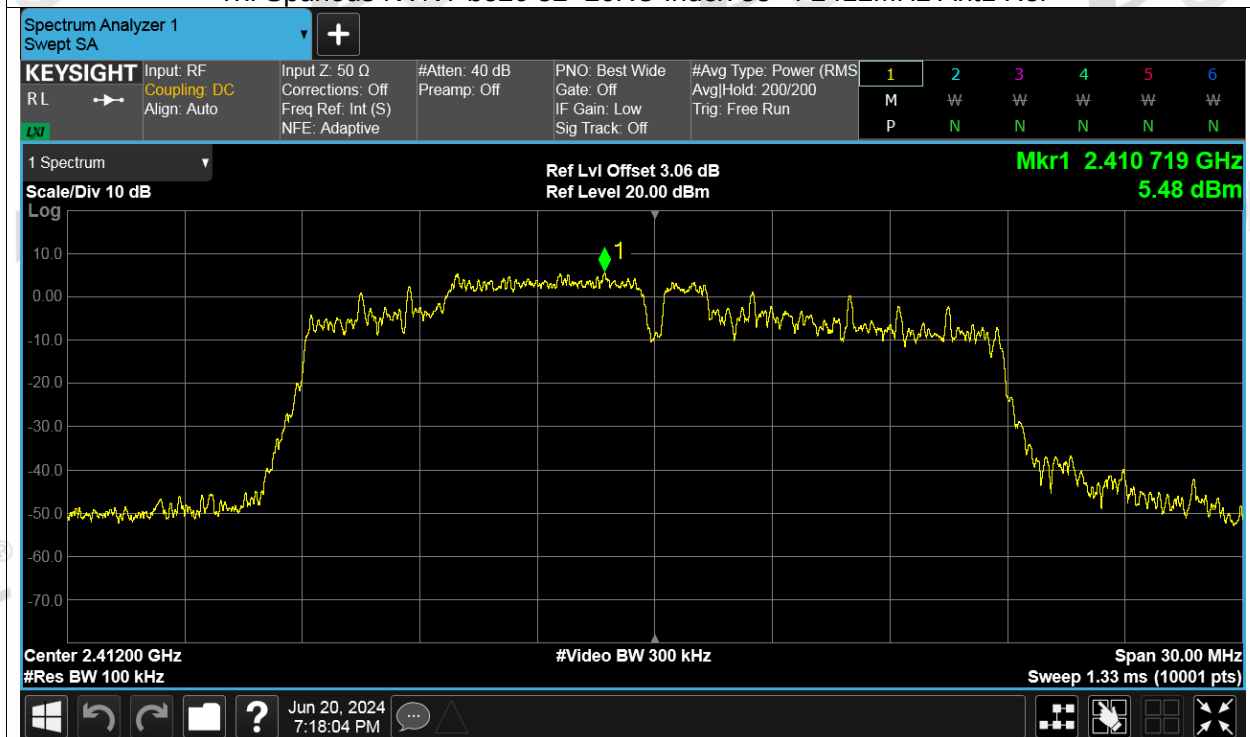
Tx. Spurious NVNT be20 52+26RU Index 38+4 2412MHz Ant1 Emission
