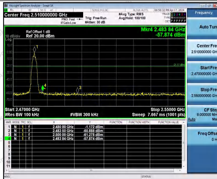
BLE_2M-Ant1-2480-PASS
