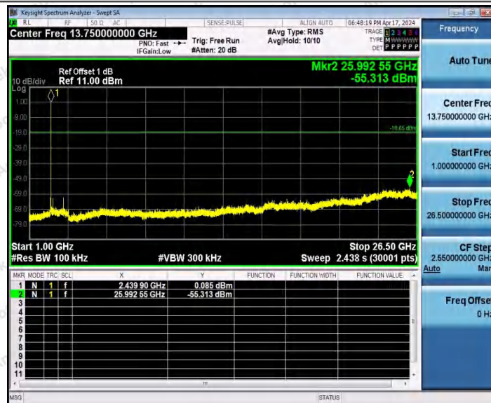
BLE_1M-Ant1-2440-1000~26500-PASS
