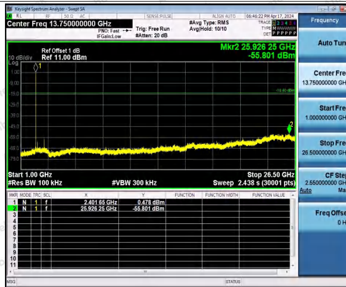
BLE_1M-Ant1-2402-1000~26500-PASS
