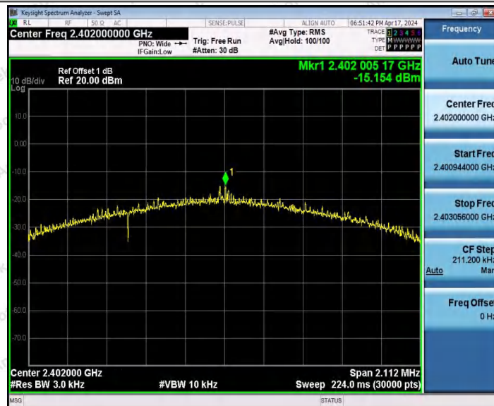
BLE_2M-Ant1-2402-PASS
