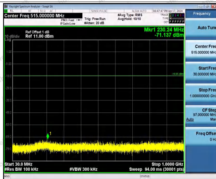
BLE_1M-Ant1-2440-30~1000-PASS
