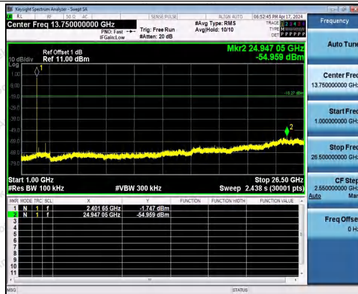
BLE_2M-Ant1-2402-1000~26500-PASS
