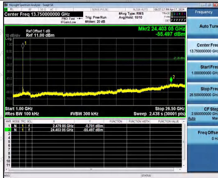
BLE_2M-Ant1-2480-1000~26500-PASS
