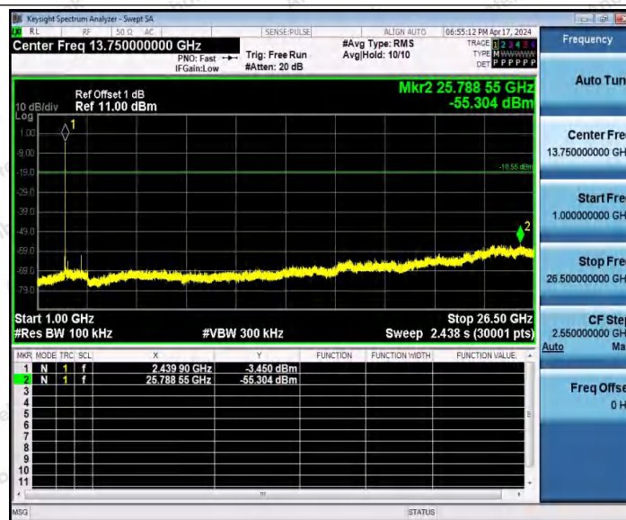
BLE_2M-Ant1-2440-1000~26500-PASS
