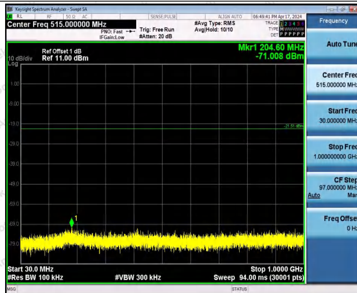
BLE_1M-Ant1-2480-30~1000-PASS
