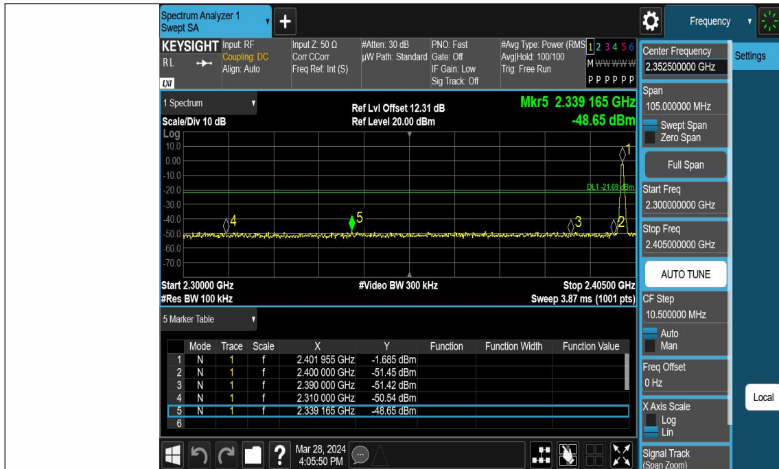
DH5-Ant1-2402-PASS
