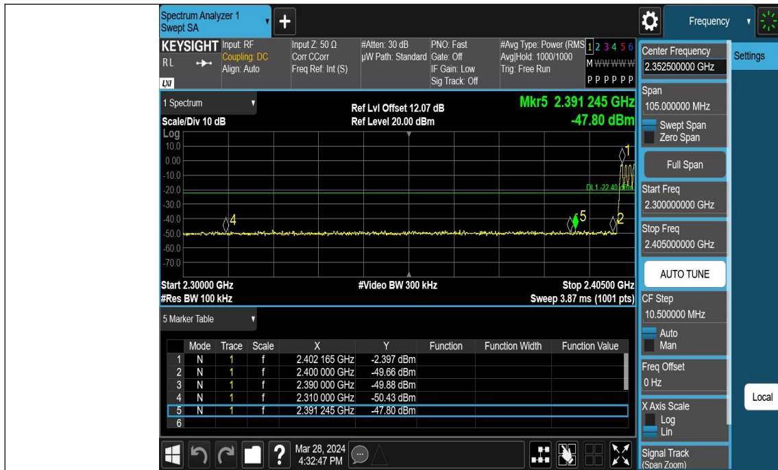
DH5-Ant1-Hop_2402-PASS
