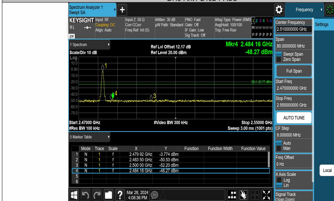
DH5-Ant1-2480-PASS
