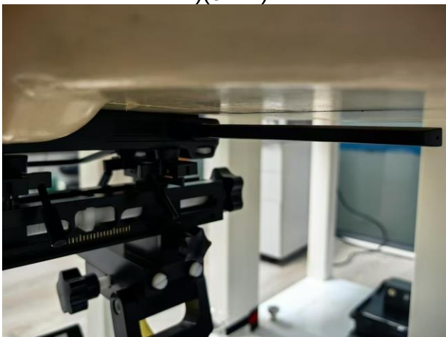
Front Horizontal mode (1g SAR for ANT 1)(0mm)
