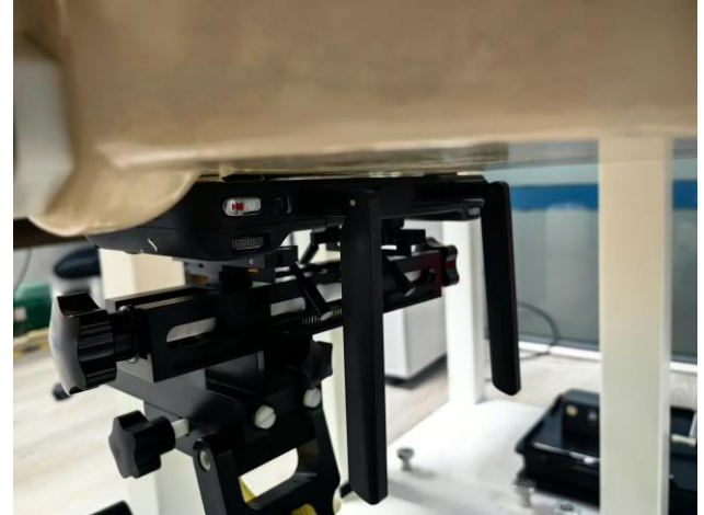
Front Vertical mode (1g SAR for ANT 2)(0mm)
