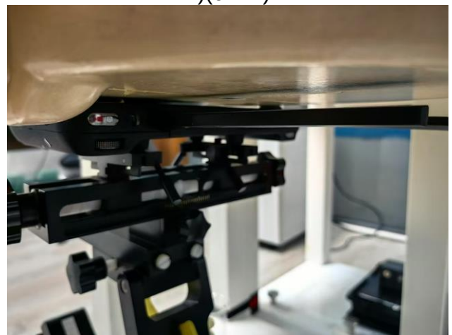
Front Horizontal mode (1g SAR for ANT 2)(0mm)
