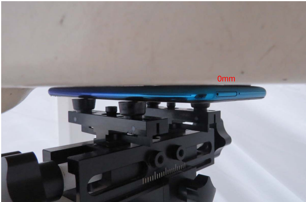
Picture 13: Back Side, the distance from handset to the bottom of the Phantom is 0mm
