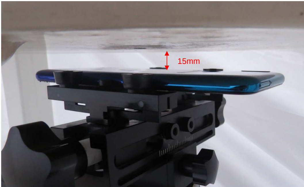
Picture 5: Back Side, the distance from handset to the bottom of the Phantom is 15mm
