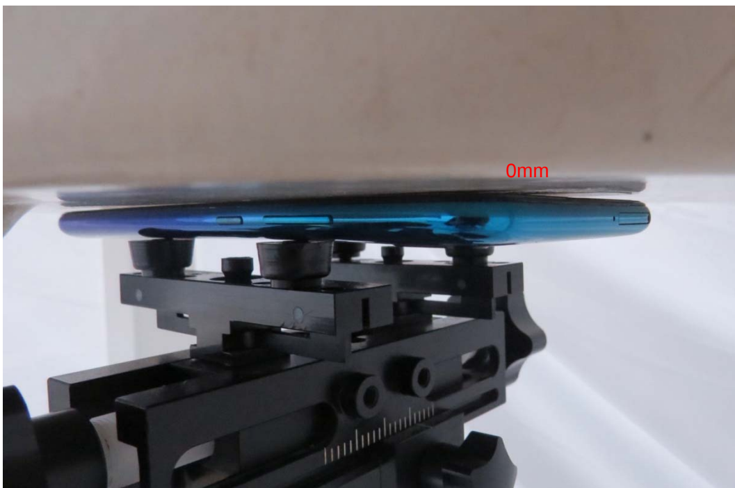
Picture 14: Front Side, the distance from handset to the bottom of the Phantom is 0mm
