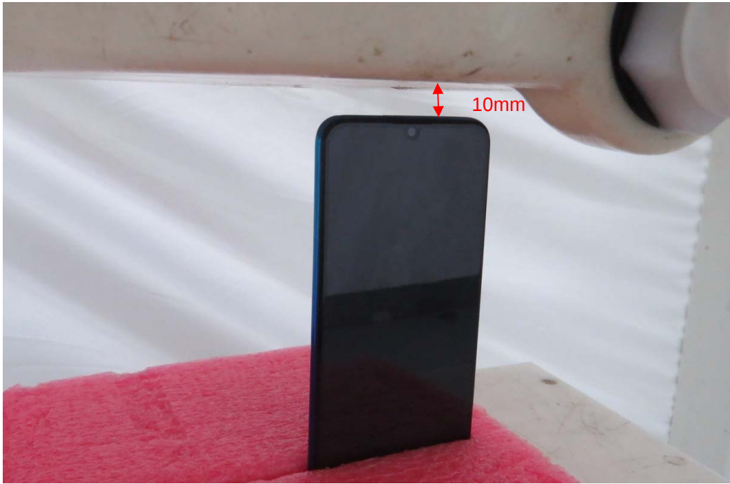
Picture 11: Top Side, the distance from handset to the bottom of the Phantom is 10mm
