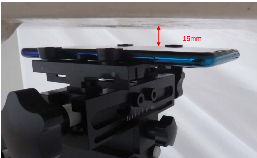
Picture 6: Front Side, the distance from handset to the bottom of the Phantom is 15mm
