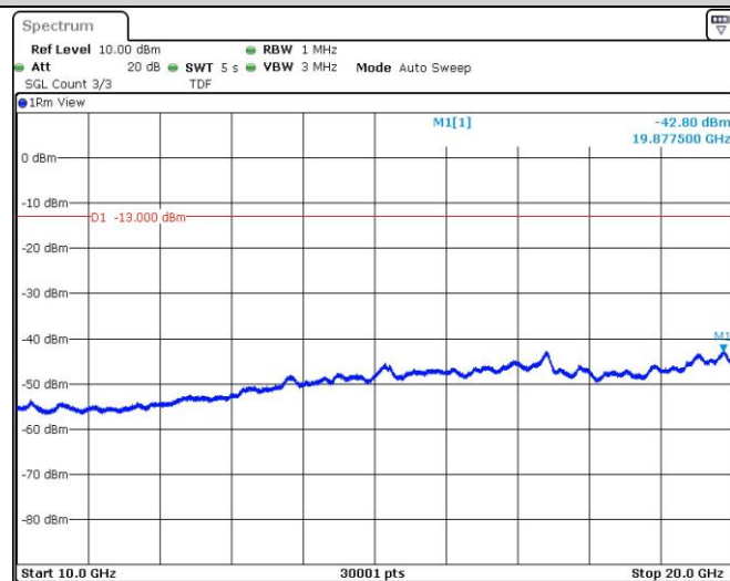
Band2-9262-3-10000~20000MHz
