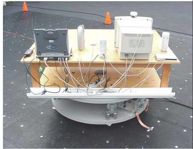
Photograph D-4 - Back of Radiated Emission Configuration
