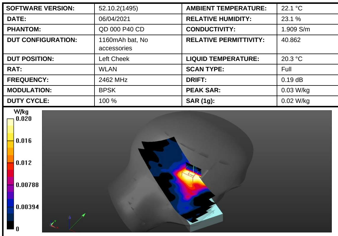
Figure 40: SAR Head Testing Results for the SC2028 at 2462 MHz.
