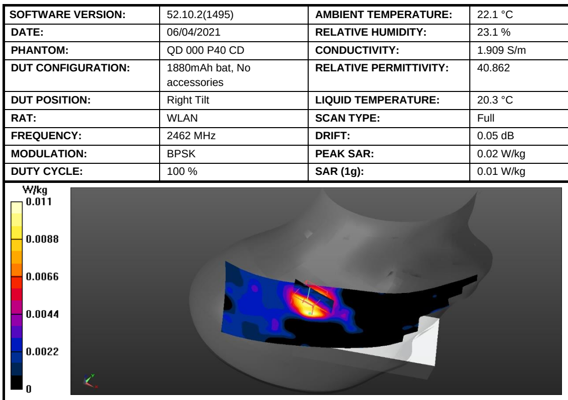
Figure 39: SAR Head Testing Results for the SC2028 at 2462 MHz.
