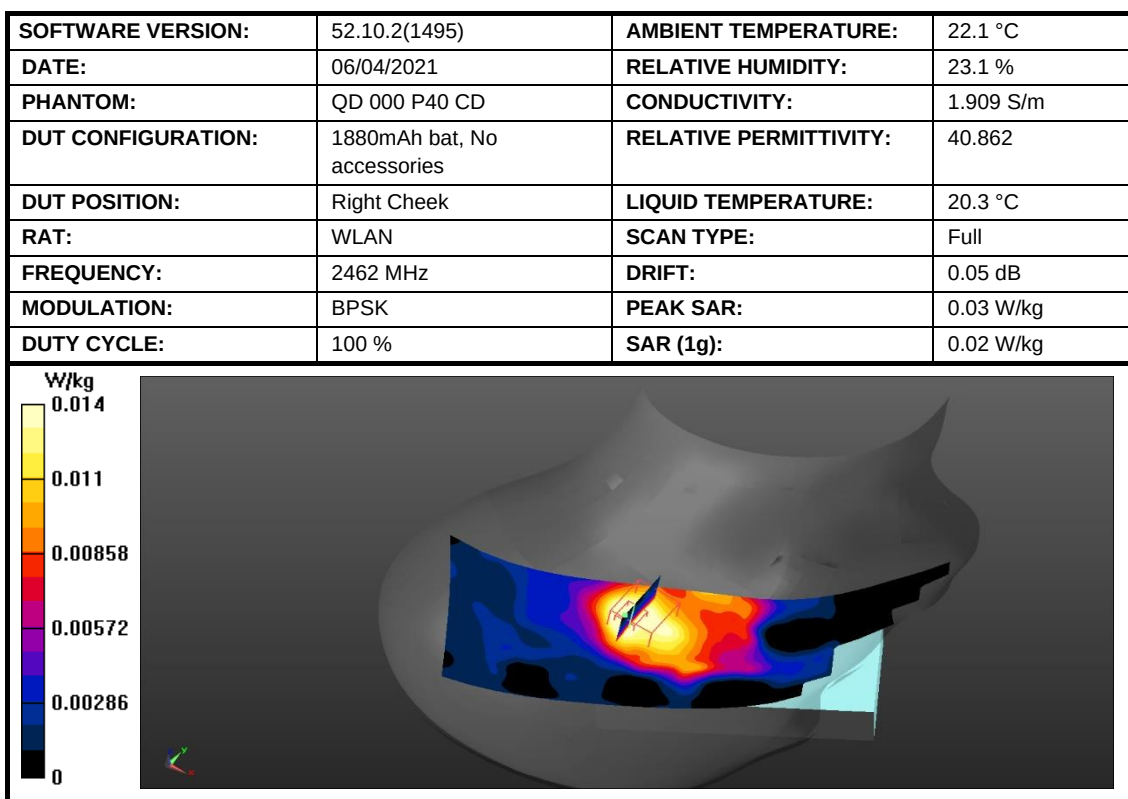
Figure 38: SAR Head Testing Results for the SC2028 at 2462 MHz.
