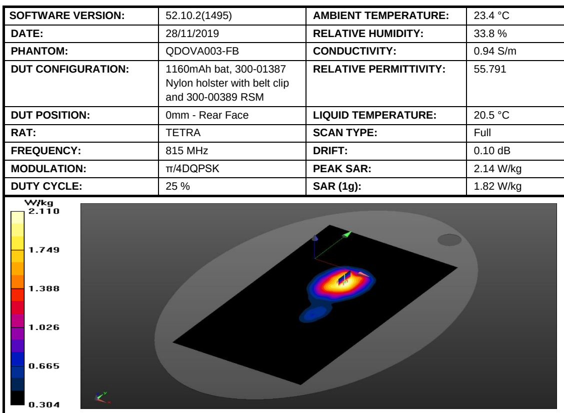
Figure 23: SAR Body Testing Results for the SC2028 at 815 MHz.
