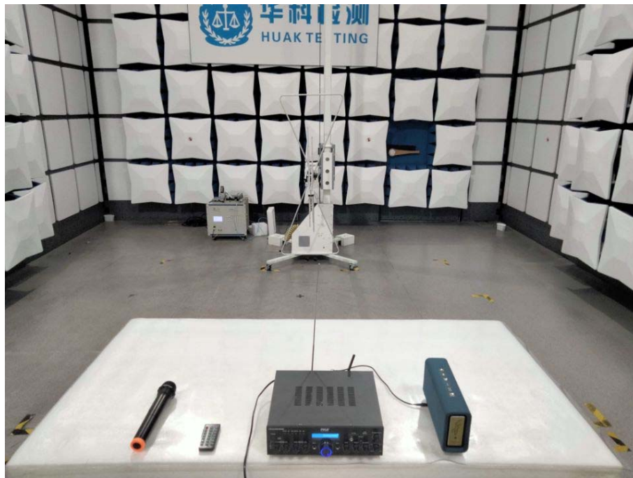
PDA8BUWM Radiated Emissions
