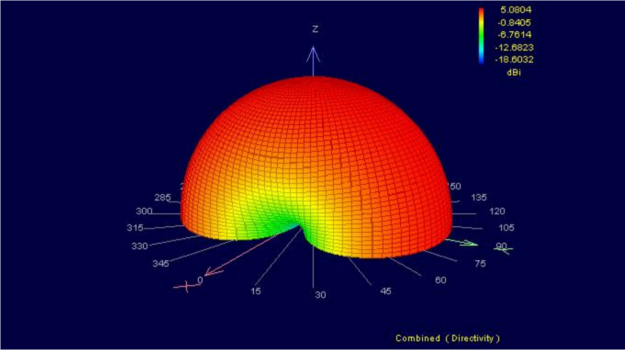
Figure 4 : 3D Far-Field Combined
