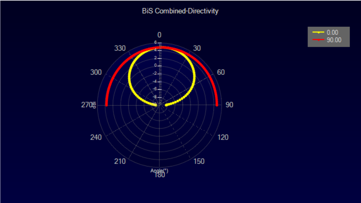
Figure 5 : Bisection Far-Field Combined
