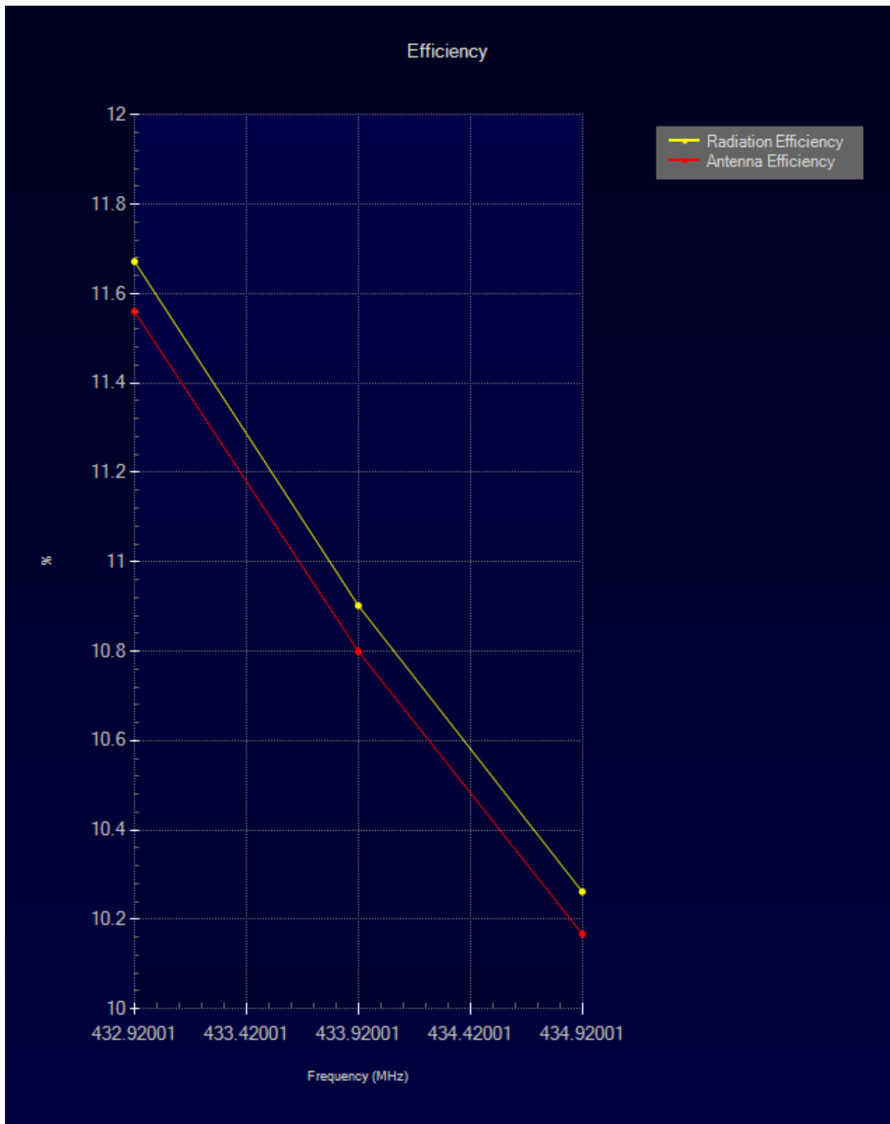
Figure 3 : Efficiency Chart
