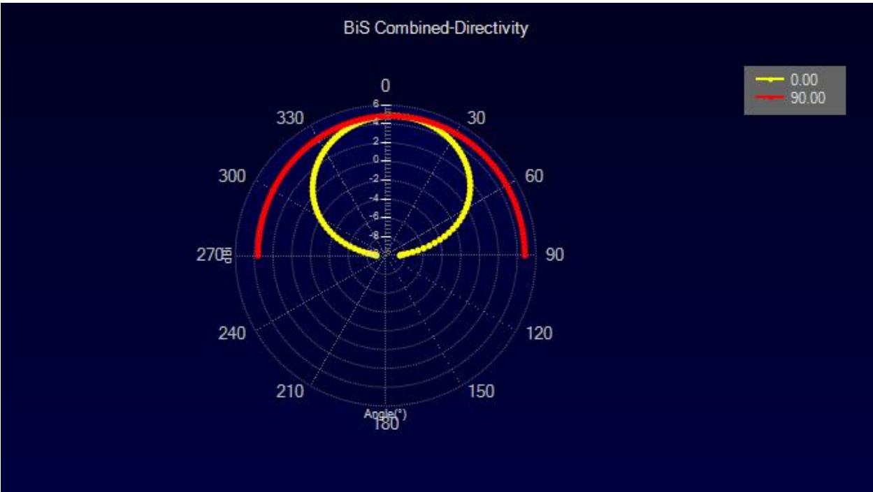
Figure 7 : Bisection Far-Field Combined
