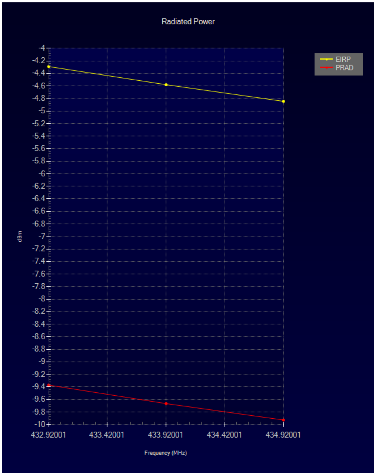
Figure 1 : Radiated Power Chart
