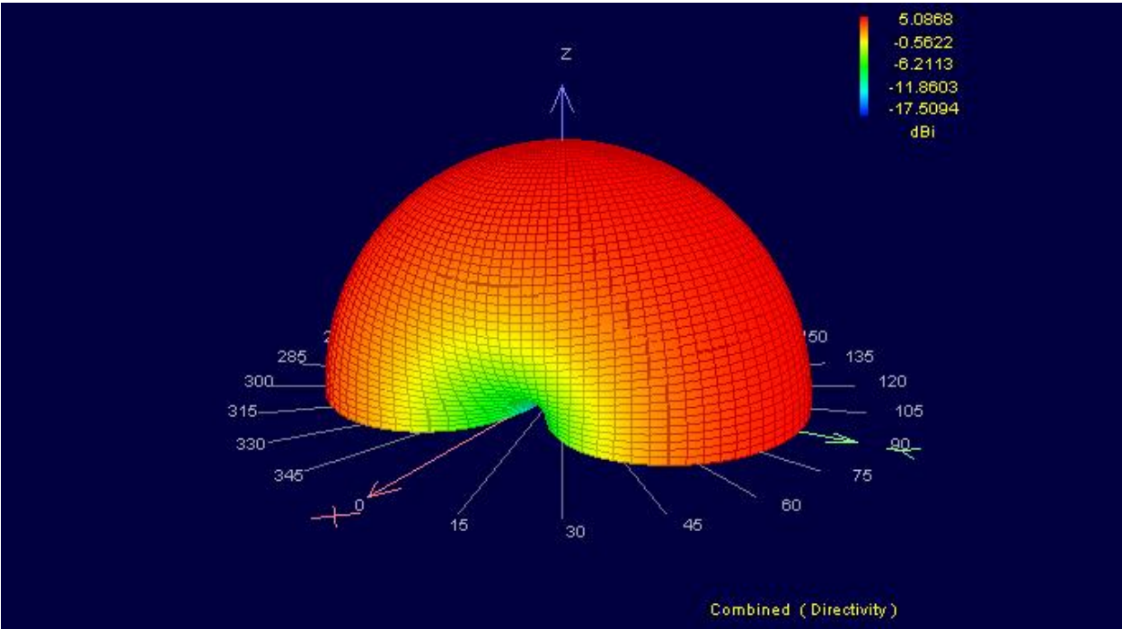
Figure 6 : 3D Far-Field Combined
