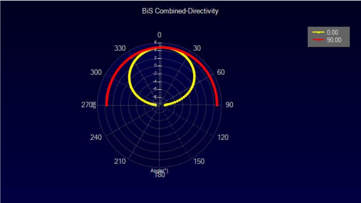
Figure 9 : Bisection Far-Field Combined
