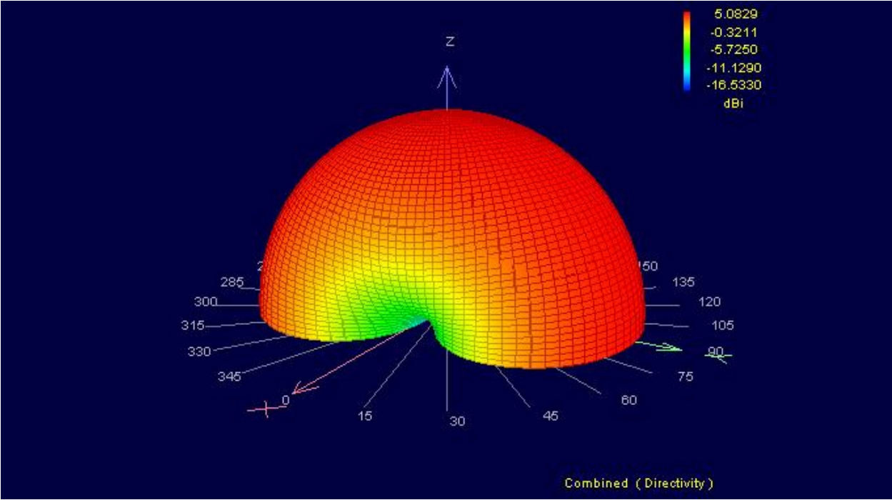
Figure 8 : 3D Far-Field Combined
