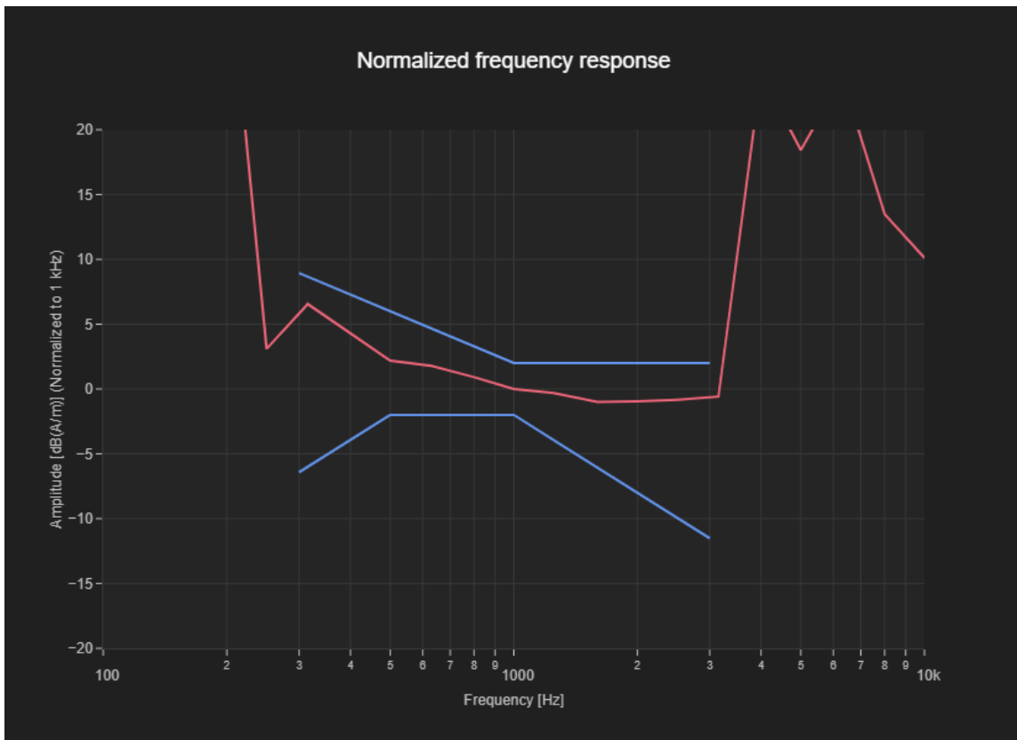
Figure C.4 Frequency Response of N78-OTT
