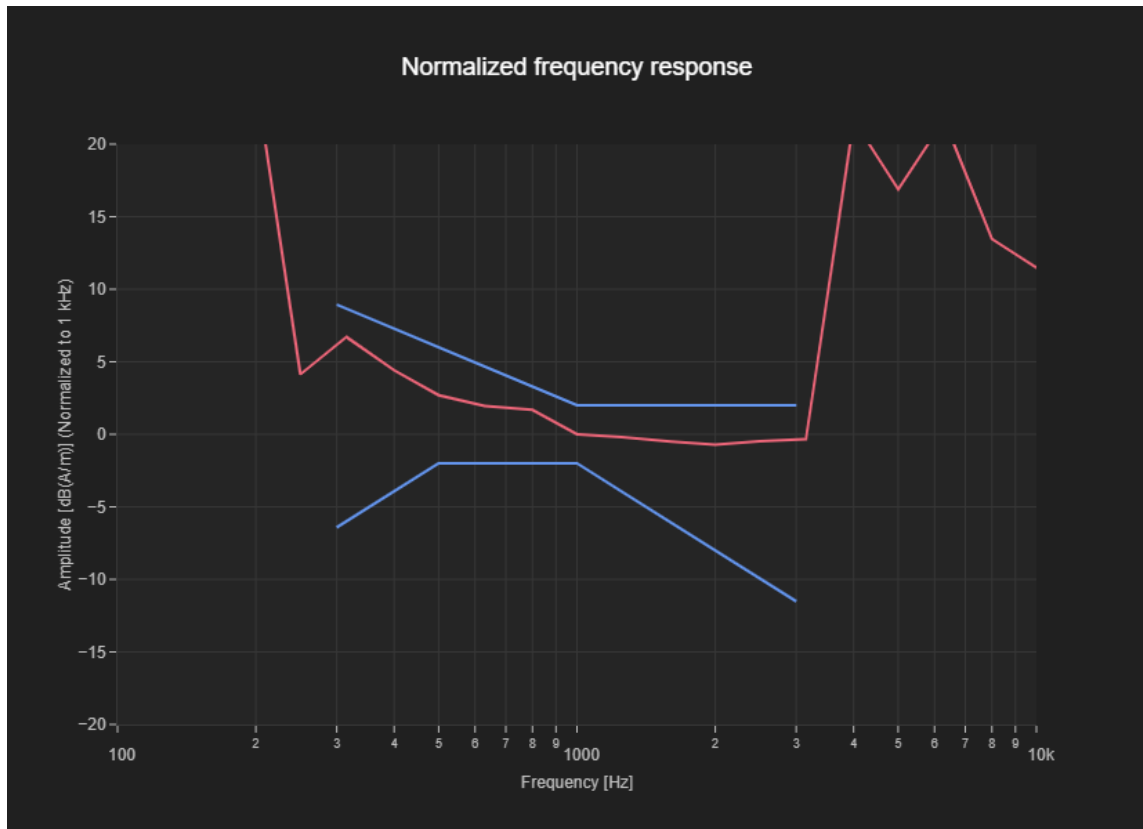
Figure C.3 Frequency Response of GSM850-OTT
