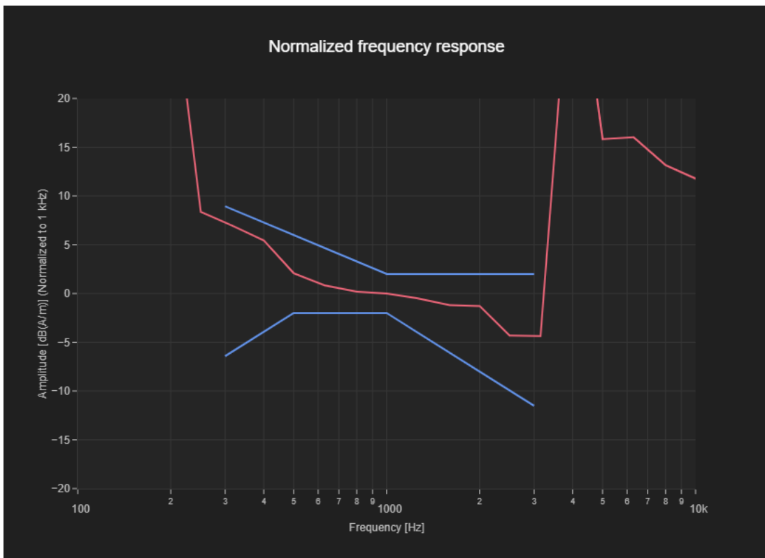
Figure C.2 Frequency Response of VoNR N78
