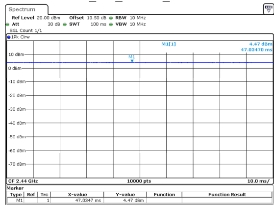
BLE_2M_Middle_Channel
