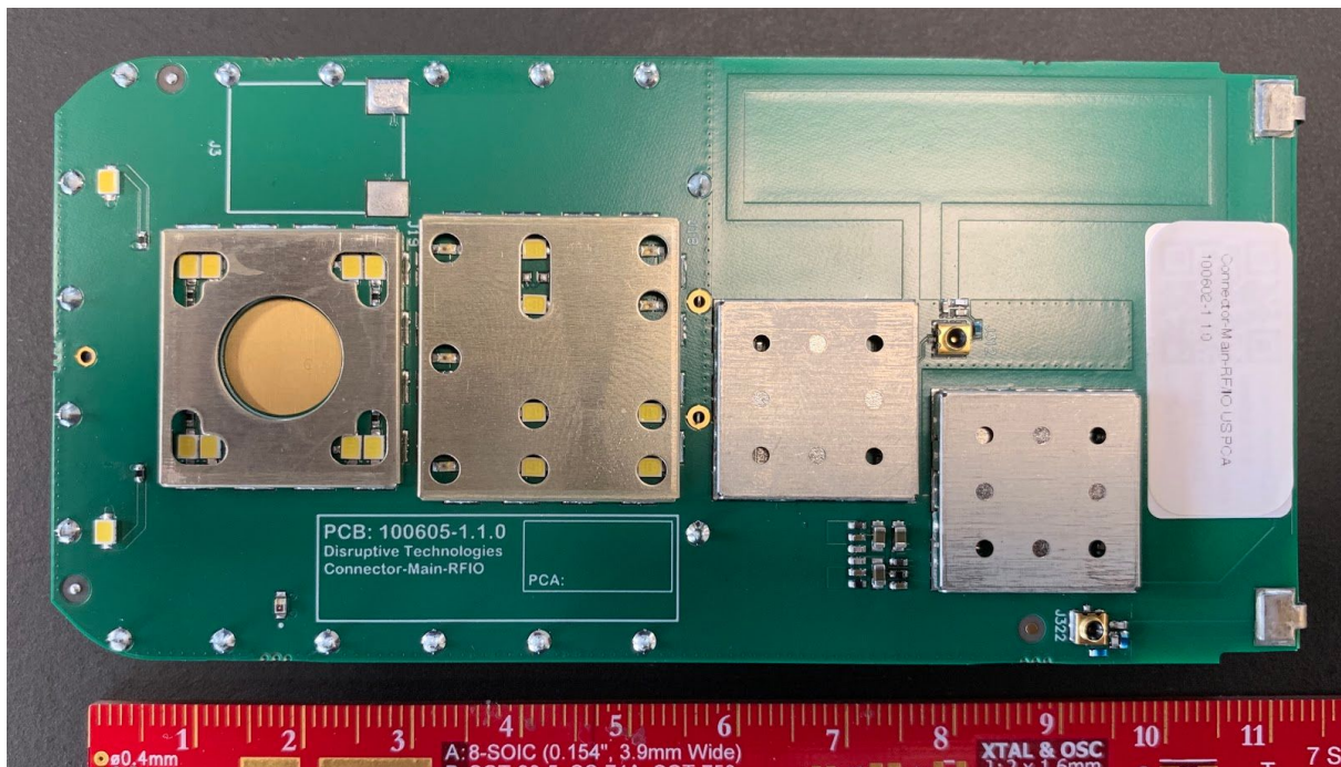
Figure 1: Picture of the top of the part 101941 DT-RFIO-Module (US)
