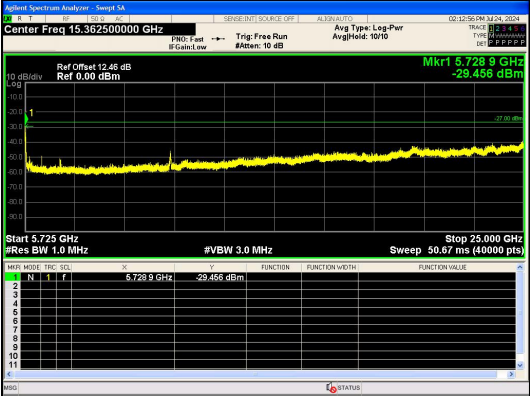
Spurious Emission:5725~25000.0 MHz IEEE 802.11ac_Channel 134_40MHz_Antenna 0
