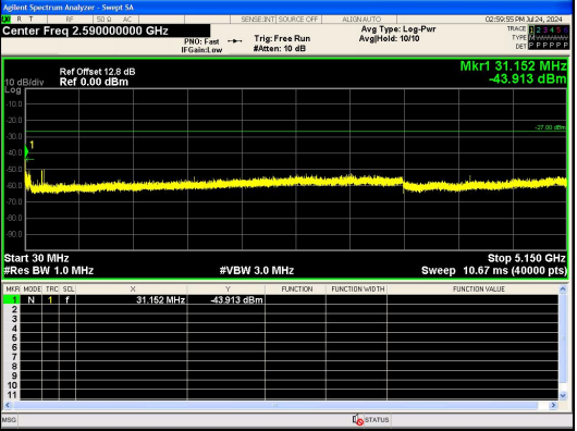
Spurious Emission:30.0~5150 MHz IEEE 802.11ac_Channel 58_80MHz_Antenna 0
