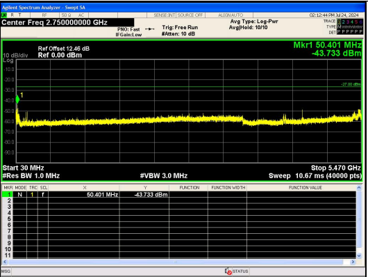
Spurious Emission:30.0~5470 MHz IEEE 802.11ac_Channel 134_40MHz_Antenna 0
