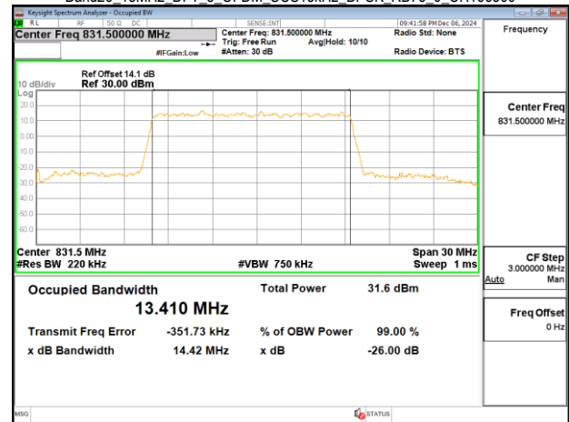
Band26 15MHz DFT s OFDM SCS15kHz BPSK RB75_0 CH167300
