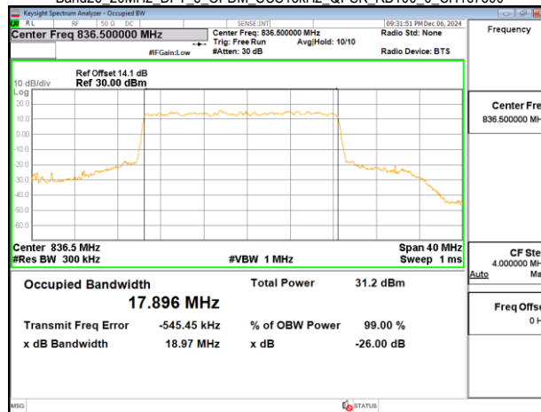
Band26 20MHz DFT s OFDM SCS15kHz QPSK RB100_0 CH167800
