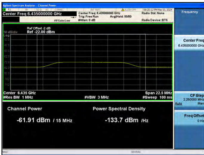
802.11ax (HE20)-Channel 97
