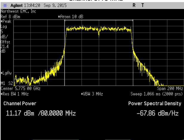
Chain C, 802.11(ac) VHT, MCS9 (256-QAM), 80 MHz, Low Channel 5775 MHz
