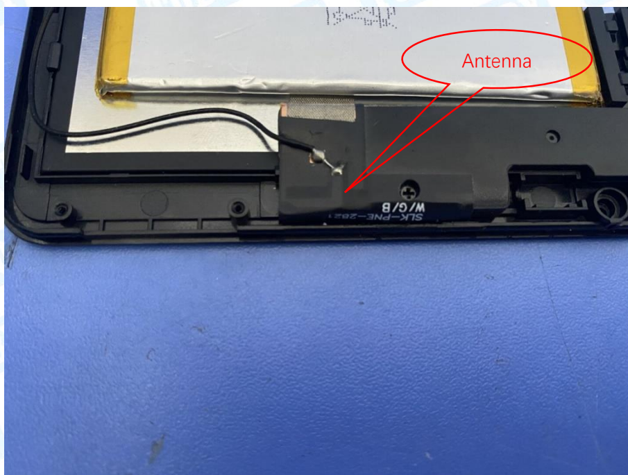
Photo 13 Internal of EUT
