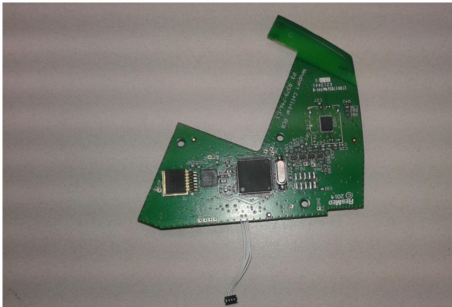
CPU side of CAM Board
