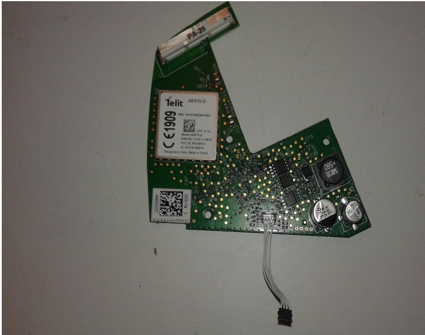
Cellular Module & Antenna Side of CAM_Board
