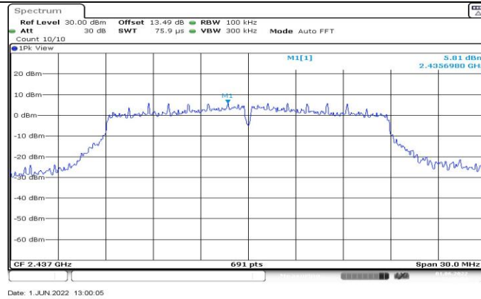
11N20SISO_Ant1_2437_0-Reference
