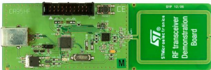
Board NFC reader
