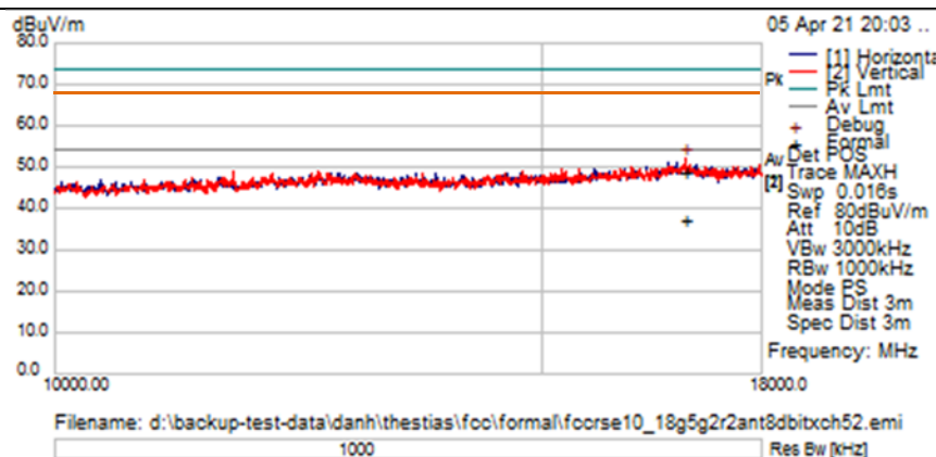
TX Spurious Emissions from 10GHz-18GHz – Ch52 (5260 MHz)
