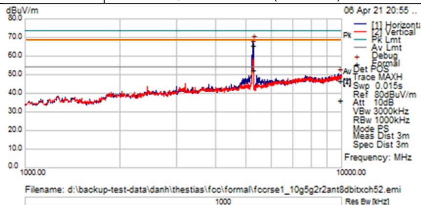
TX Spurious Emissions from 1GHz-10GHz – Ch52 (5260 MHz)
