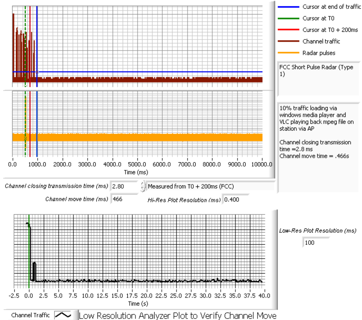
Radar Type 1 FCC Closing and Moving time plot
