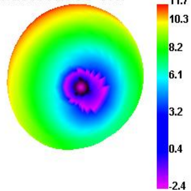
Bluetooth 78 TRP
