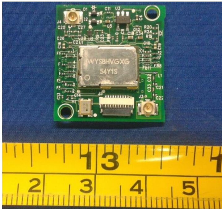
EUT Radio with Shielding Top View
