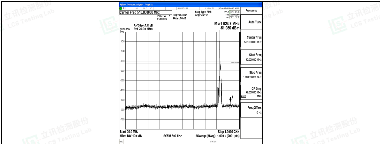
Band5_10MHz_16QAM_20525_1RB#0_30~1000_30~1000
