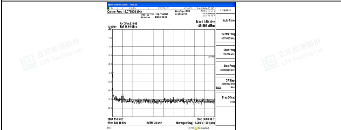
Band5_10MHz_16QAM_20525_1RB#0_0.15~30_0.15~30
