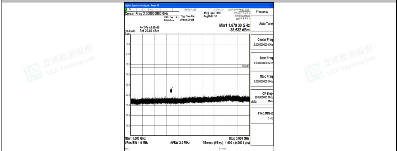
Band5_10MHz_16QAM_20600_1RB#0_1000~3000_1000~3000
