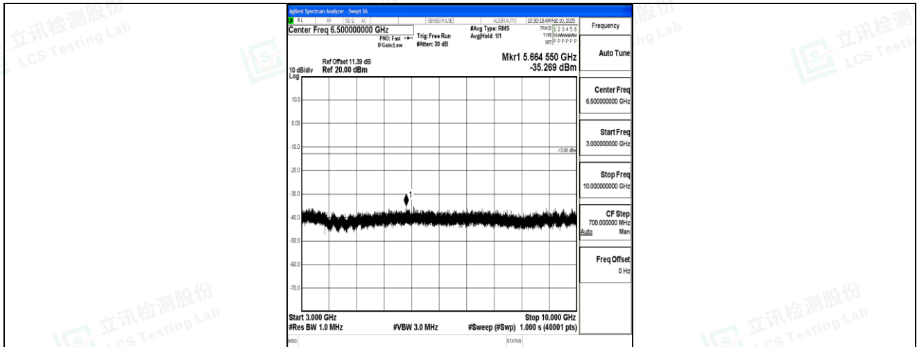
Band5_5MHz_16QAM_20625_1RB#0_3000~10000_3000~10000
