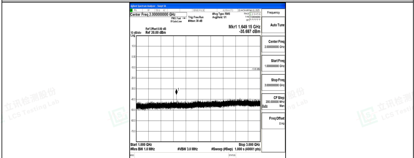
Band5_10MHz_QPSK_20450_1RB#0_1000~3000_1000~3000
