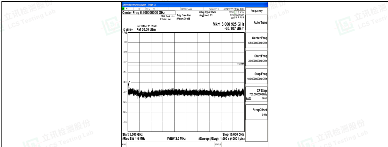
Band5_10MHz_QPSK_20525_1RB#0_3000~10000_3000~10000
