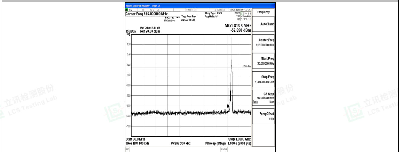
Band5_10MHz_16QAM_20600_1RB#0_30~1000_30~1000
