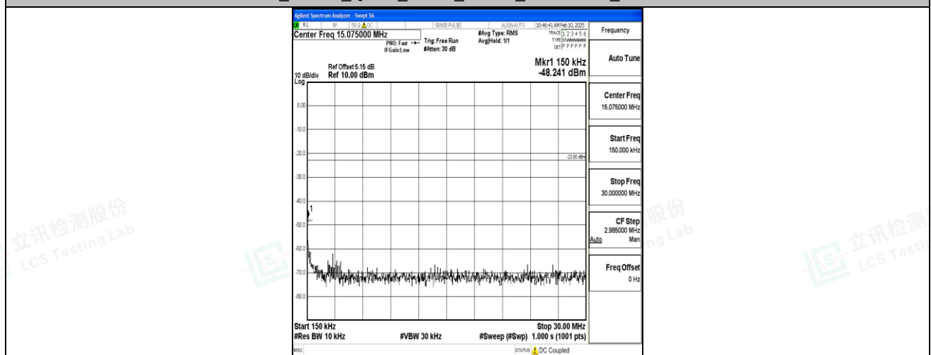
Band5_10MHz_QPSK_20600_1RB#0_0.15~30_0.15~30
