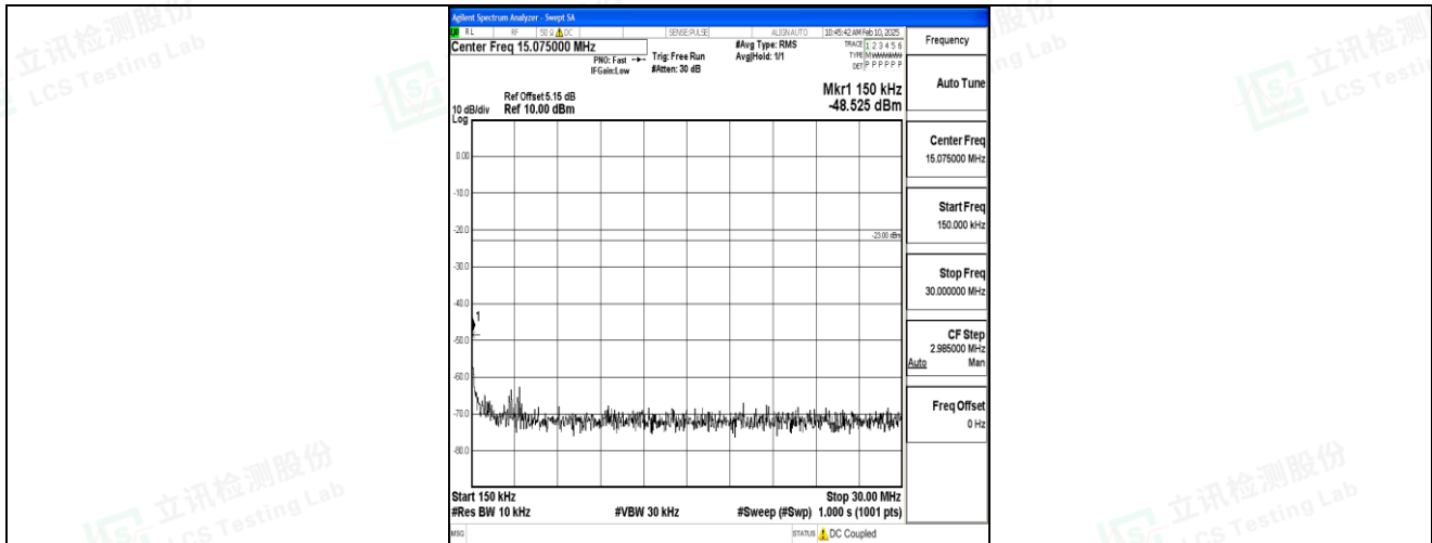
Band5_10MHz_QPSK_20525_1RB#0_0.15~30_0.15~30
