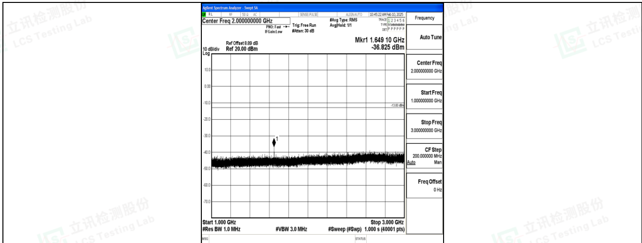
Band5_10MHz_16QAM_20450_1RB#0_1000~3000_1000~3000
