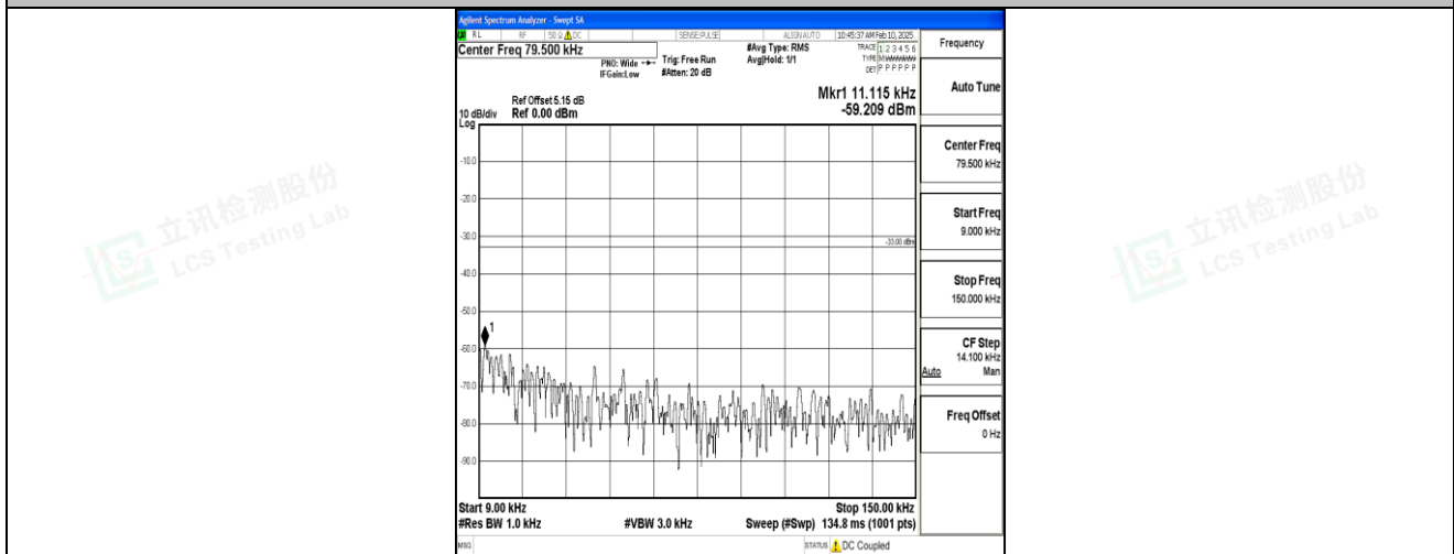
Band5_10MHz_QPSK_20525_1RB#0_0.009~0.15_0.009~0.15
