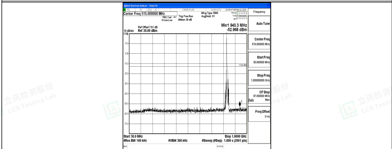
Band5_10MHz_QPSK_20525_1RB#0_30~1000_30~1000
