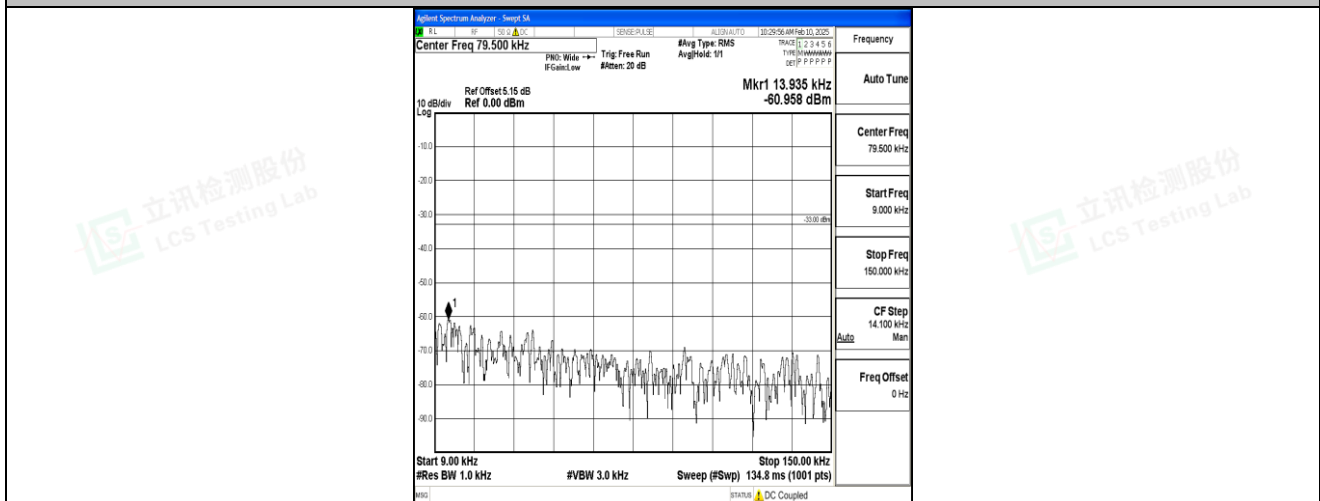
Band5_5MHz_16QAM_20625_1RB#0_0.009~0.15_0.009~0.15
