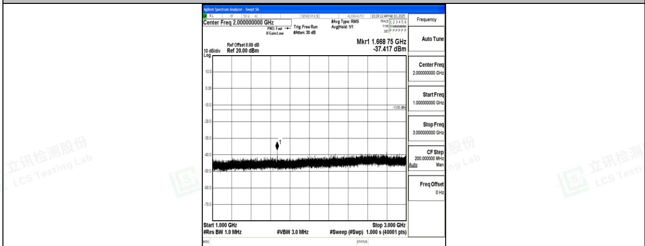
Band5_5MHz_16QAM_20525_1RB#0_1000~3000_1000~3000
