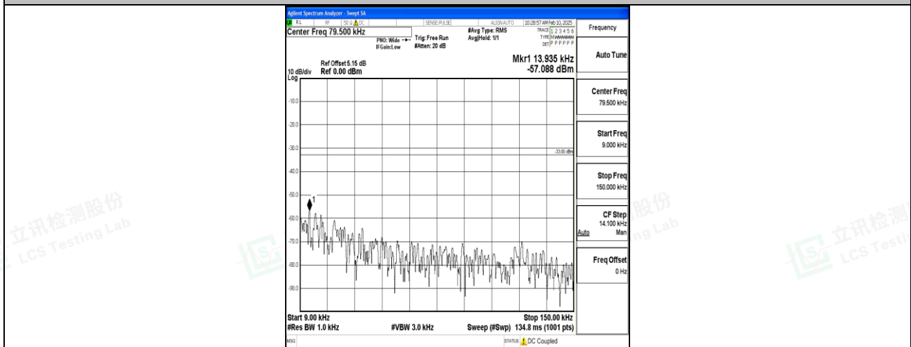
Band5_5MHz_16QAM_20525_1RB#0_0.009~0.15_0.009~0.15
