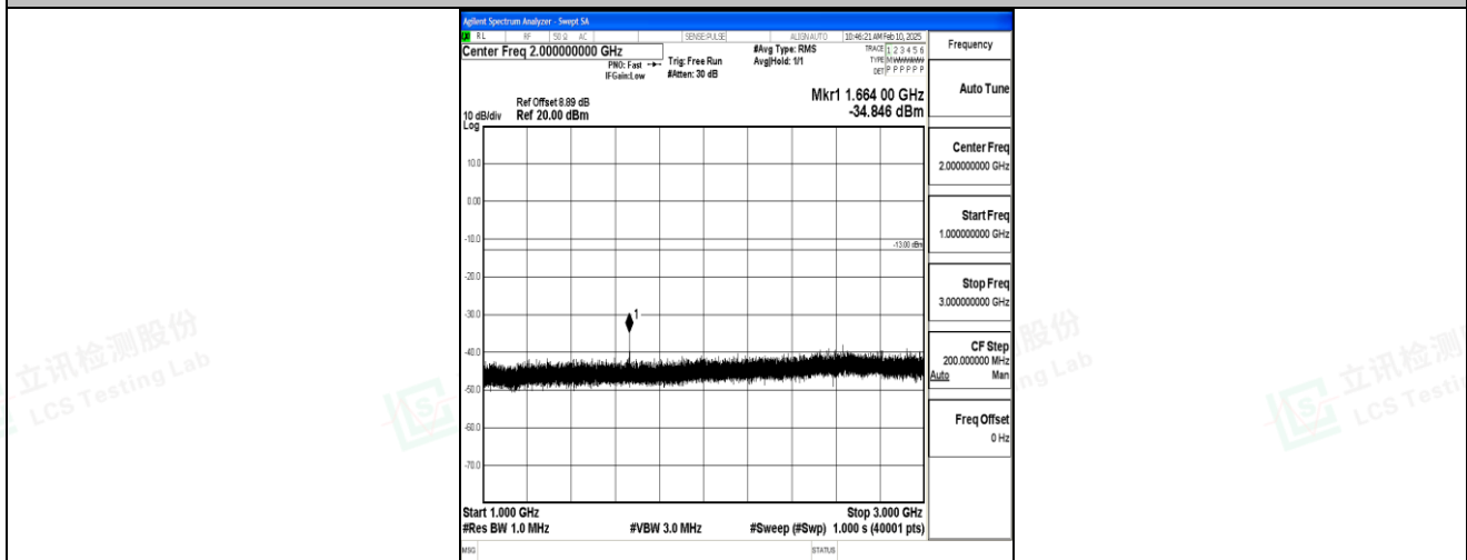
Band5_10MHz_16QAM_20525_1RB#0_1000~3000_1000~3000
