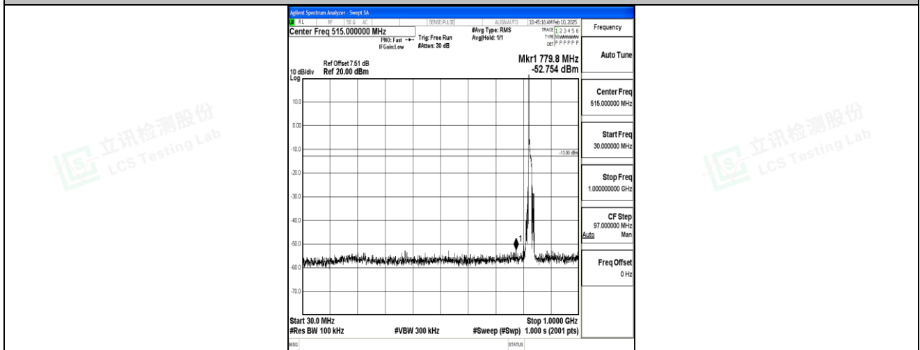
Band5_10MHz_16QAM_20450_1RB#0_30~1000_30~1000
