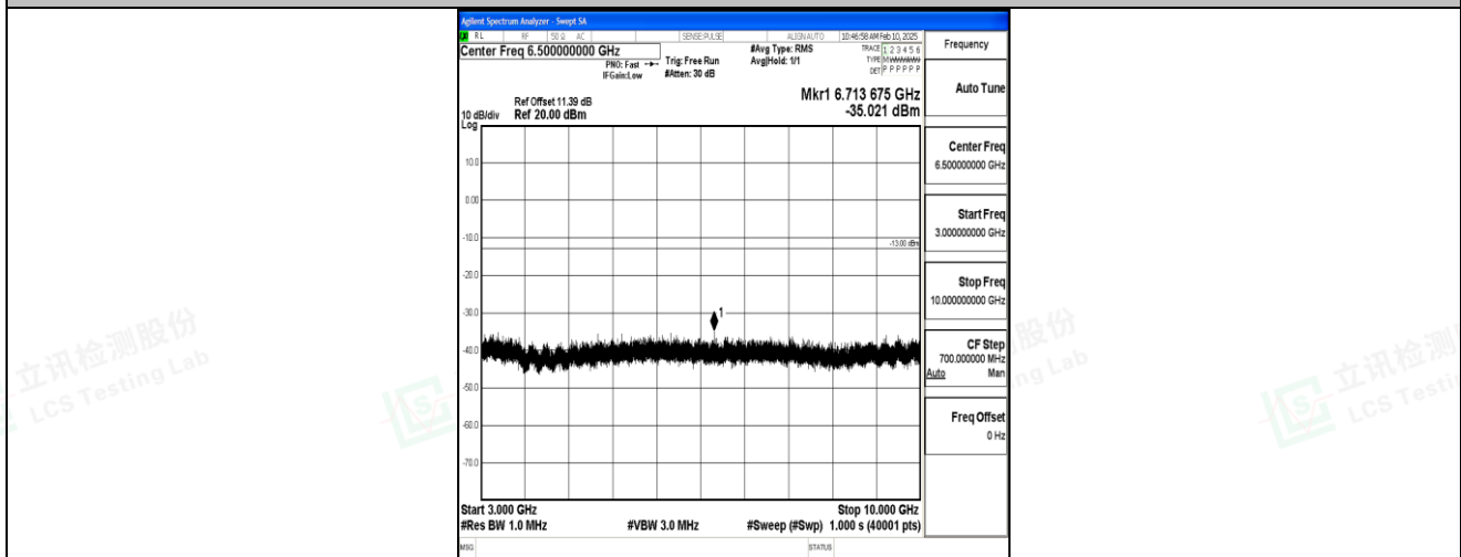
Band5_10MHz_QPSK_20600_1RB#0_3000~10000_3000~10000
