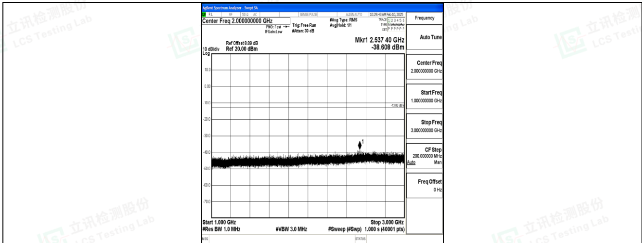
Band5_5MHz_QPSK_20625_1RB#0_1000~3000_1000~3000
