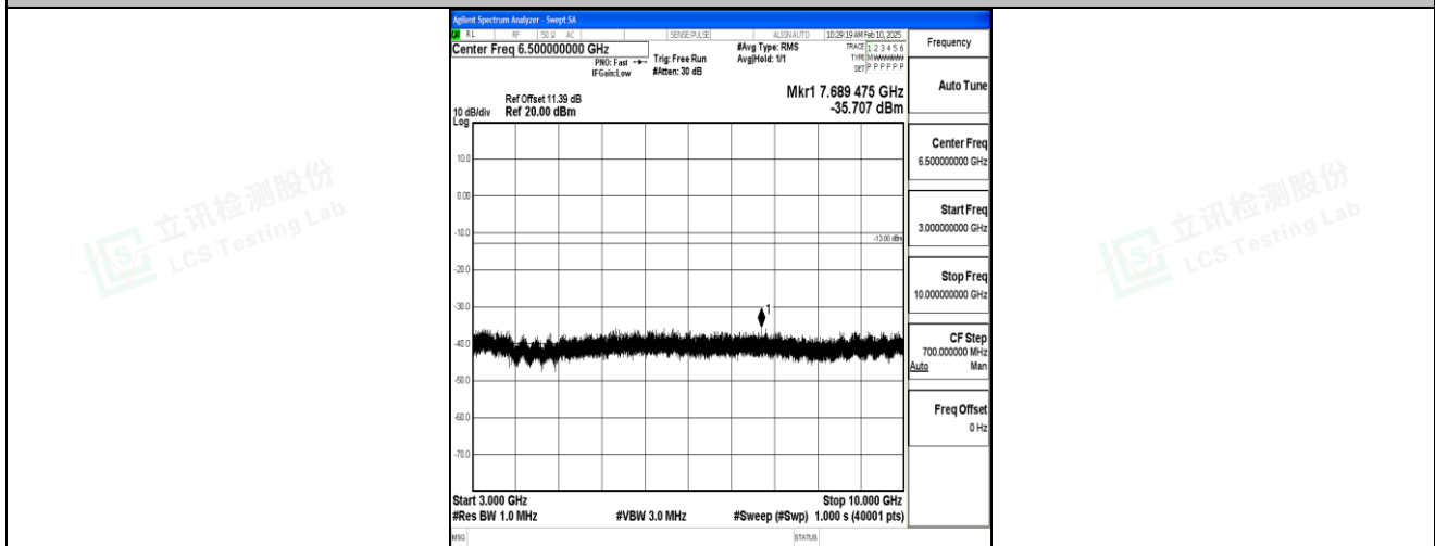
Band5_5MHz_16QAM_20525_1RB#0_3000~10000_3000~10000
