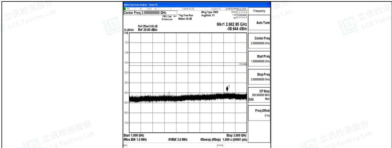
Band5_10MHz_QPSK_20600_1RB#0_1000~3000_1000~3000
