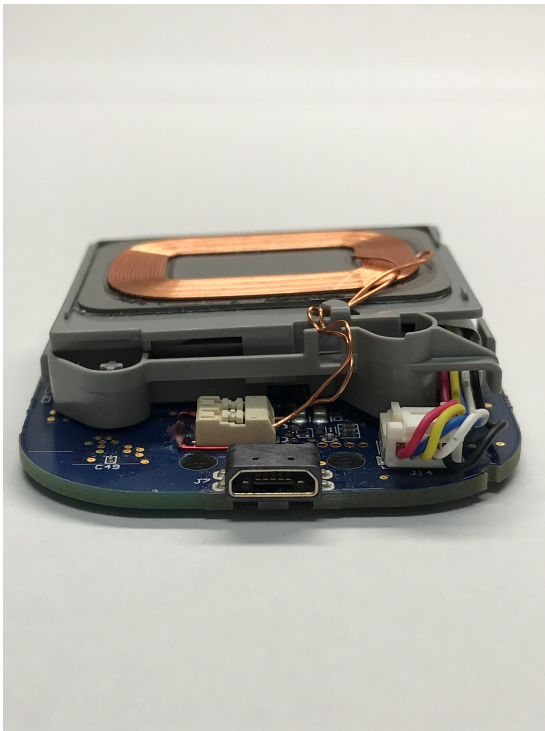
Figure 12: Communicator, Model TM91, Hybrid Inside Housing Side View
