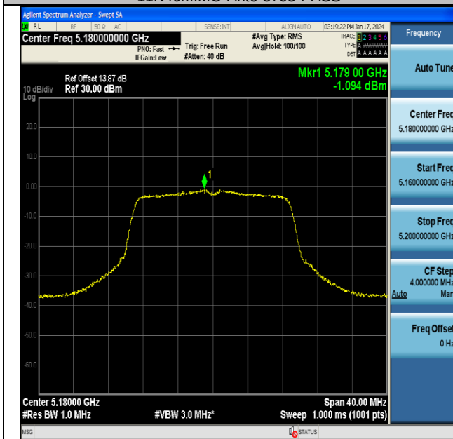
11AC20MIMO-Ant6-5180-PASS
