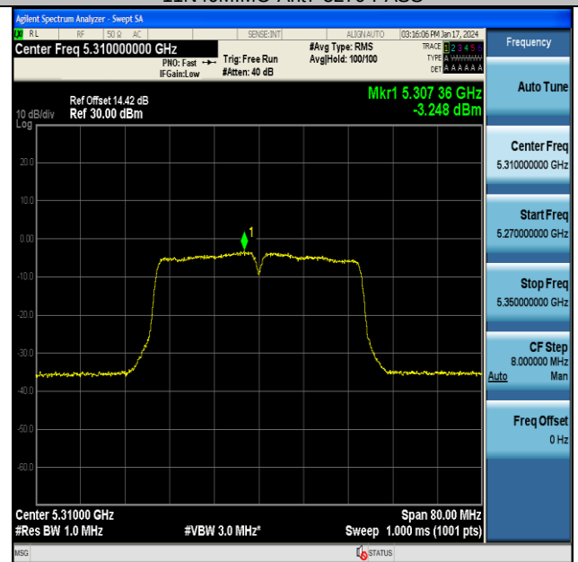
11N40MIMO-Ant7-5310-PASS
