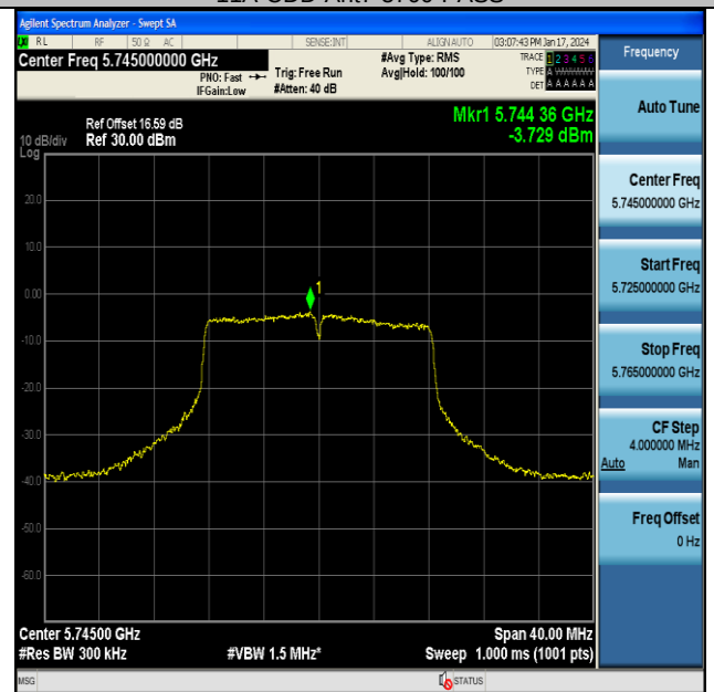
11A-CDD-Ant7-5745-PASS
