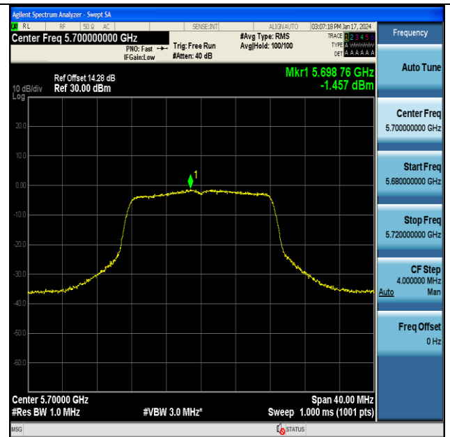
11A-CDD-Ant7-5700-PASS
