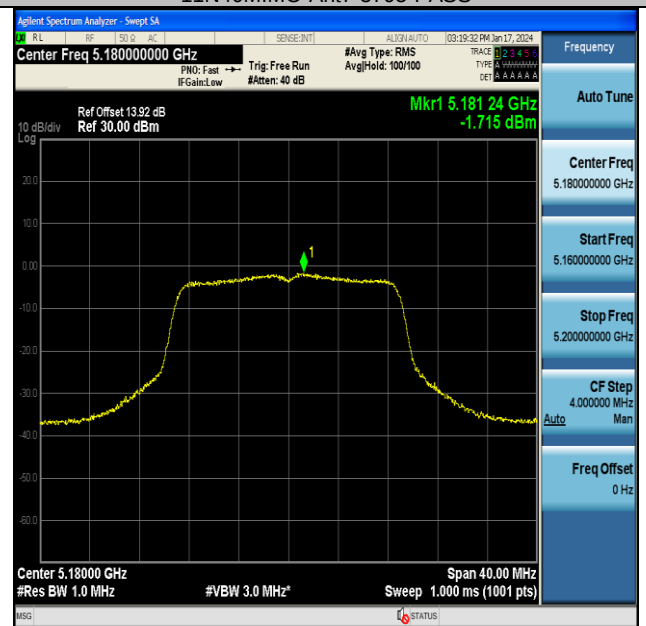
11AC20MIMO-Ant7-5180-PASS
