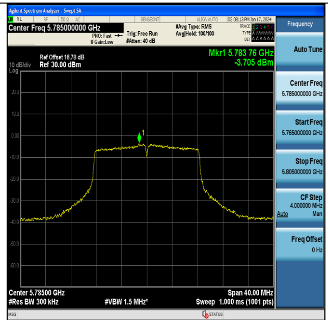
11A-CDD-Ant7-5785-PASS
