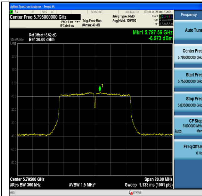
11N40MIMO-Ant6-5795-PASS
