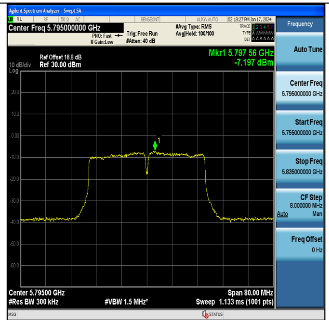
11N40MIMO-Ant7-5795-PASS
