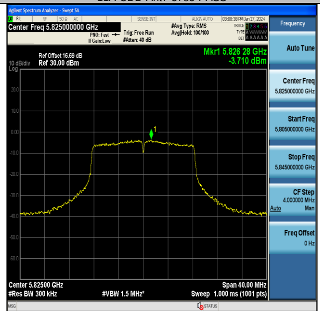
11A-CDD-Ant7-5825-PASS
