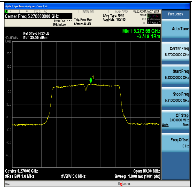
11N40MIMO-Ant7-5270-PASS
