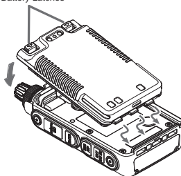
Battery Latches
