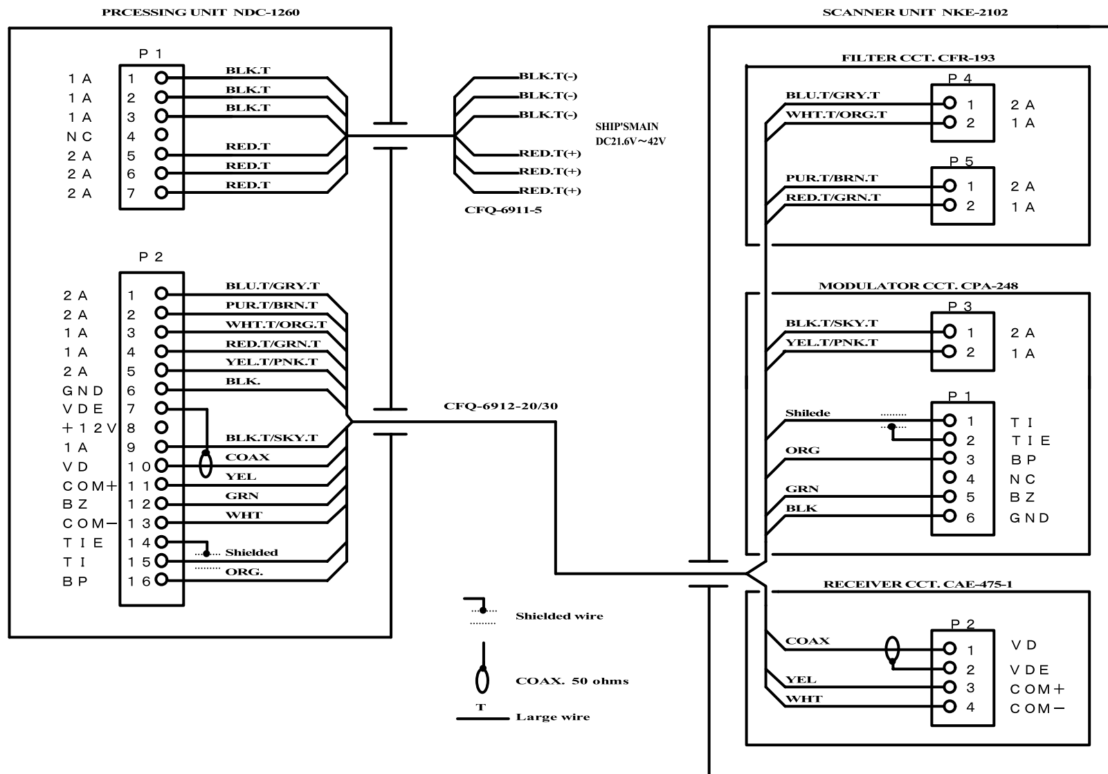
[Fig. 103 INTERCONNECTION DIAGRAM OF JMA-5110]
