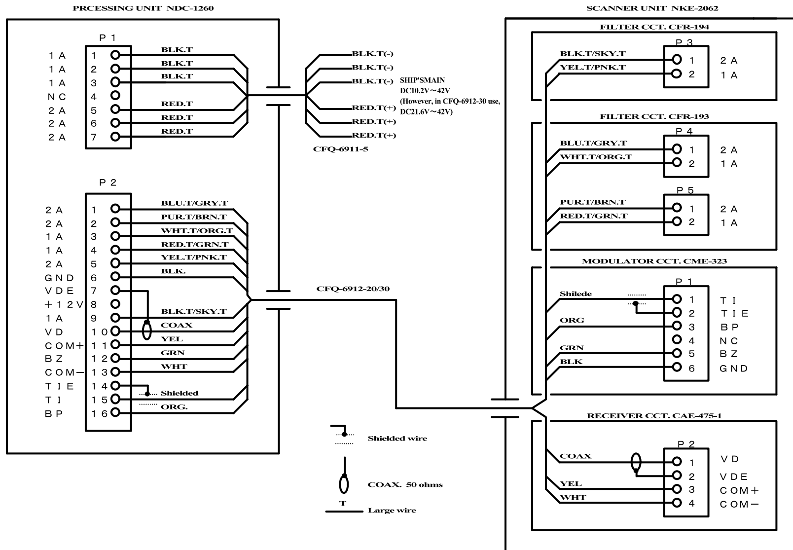
[Fig. 102 INTERCONNECTION DIAGRAM OF JMA-5106]
