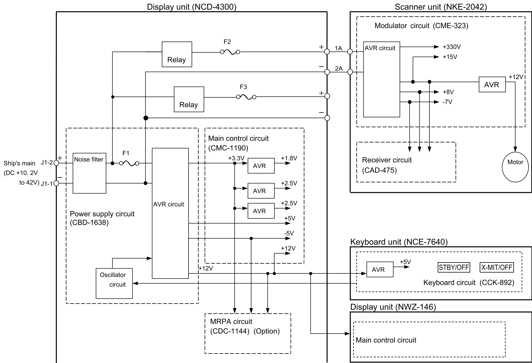
[Fig. 104. PRIMARY POWER SYSTEM DIAGRAM OF JMA-5104]
