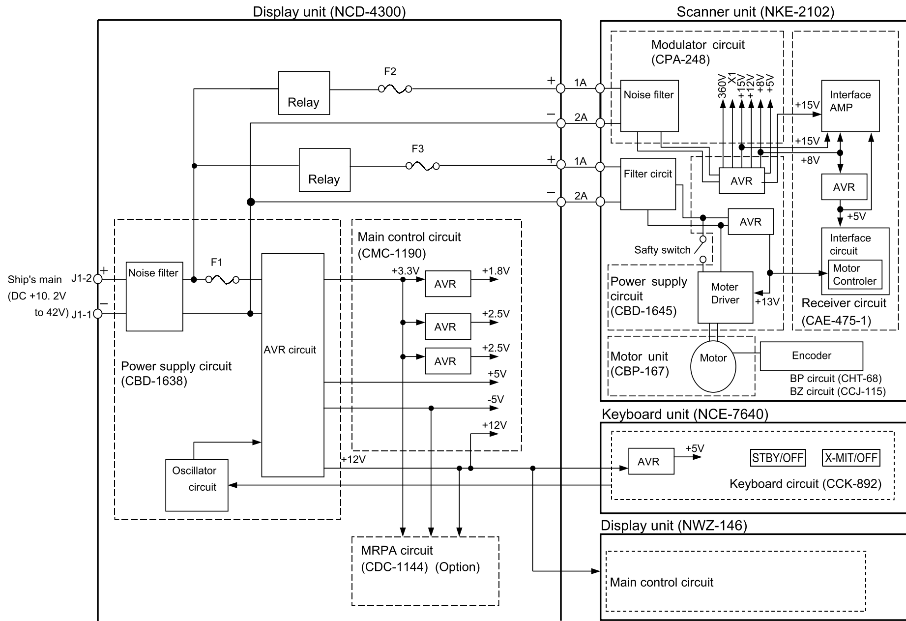
[Fig. 106 PRIMARY POWER SYSTEM DIAGRAM OF JMA-5110]
