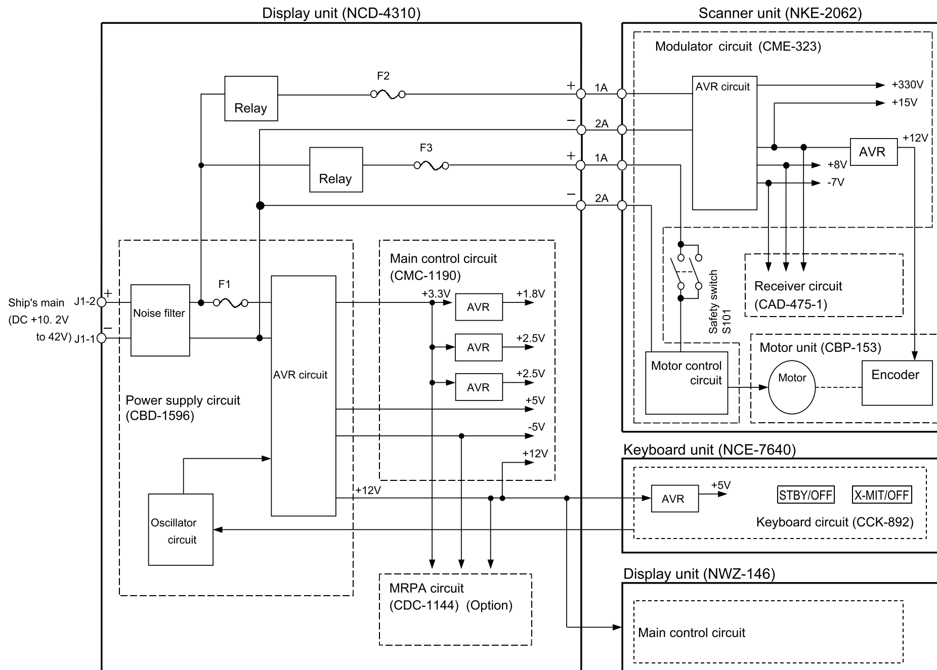
[Fig. 105 PRIMARY POWER SYSTEM DIAGRAM OF JMA-5106]
