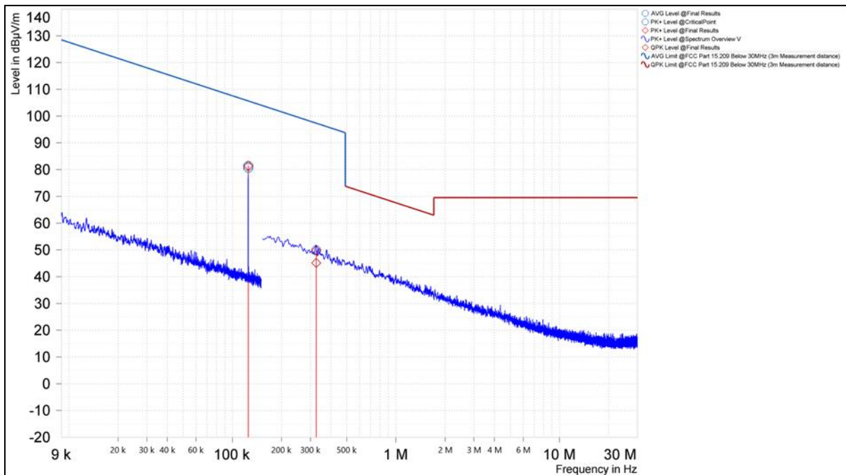
Figure 7. Spurious Emissions Below 30MHz, (LF Antenna, Coaxial Loop)
