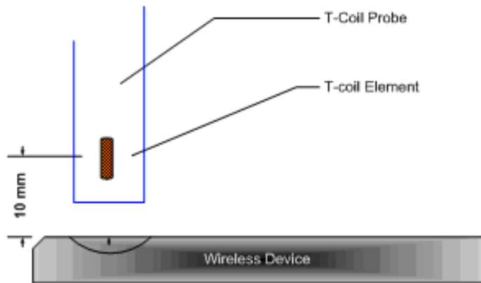
Figure 5-10 Measurement Distance
