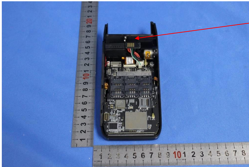
2G4G antenna
