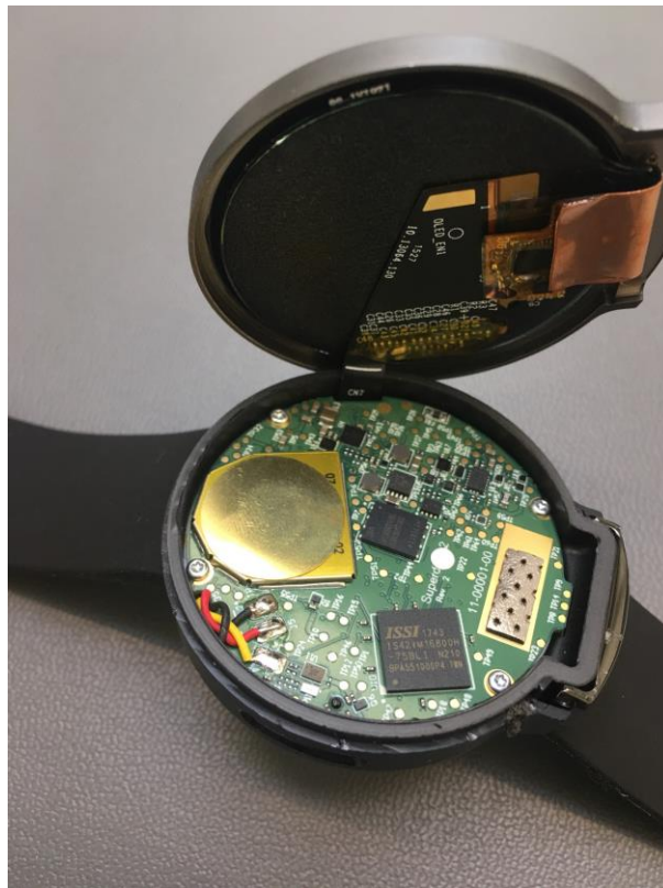
Figure 2 MainBoard
