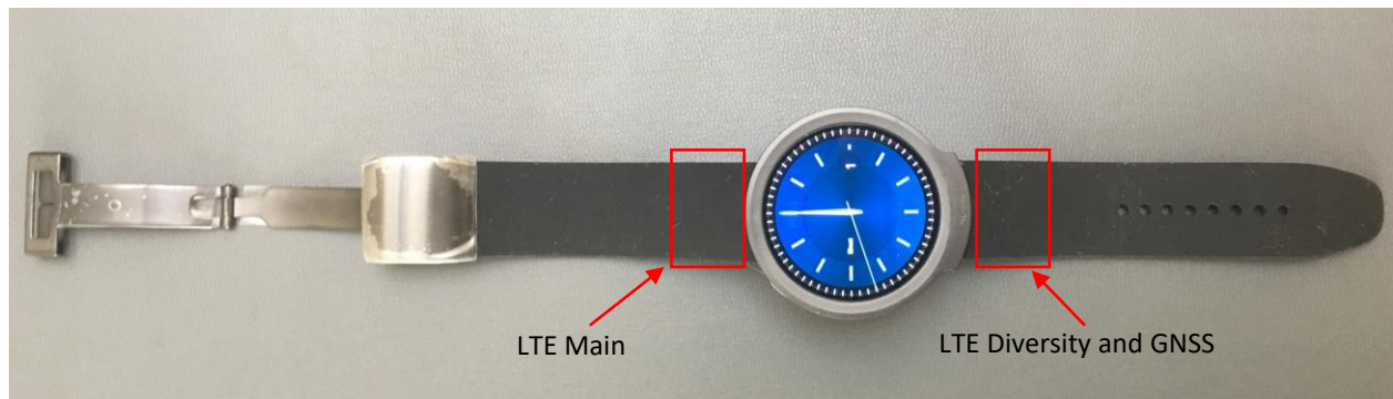
Figure 1 Heart Watch Antenna Location. Antennas are overmolded into the Straps
