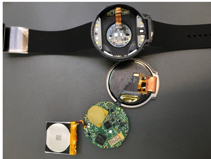
Figure 4 MainBoard and Battery removed.
