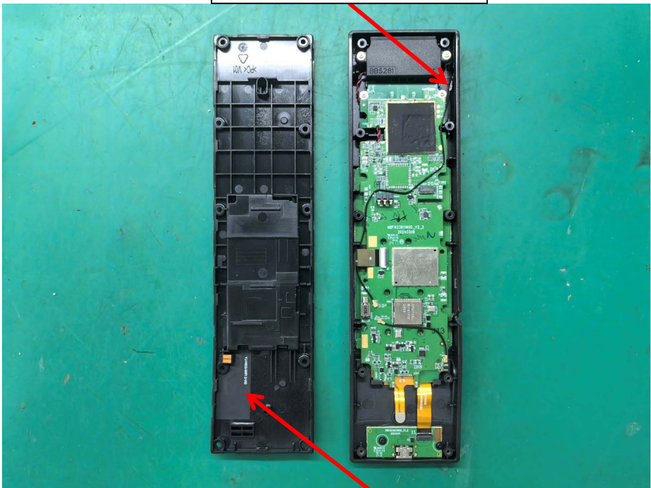
WiFi 2 Antenna
