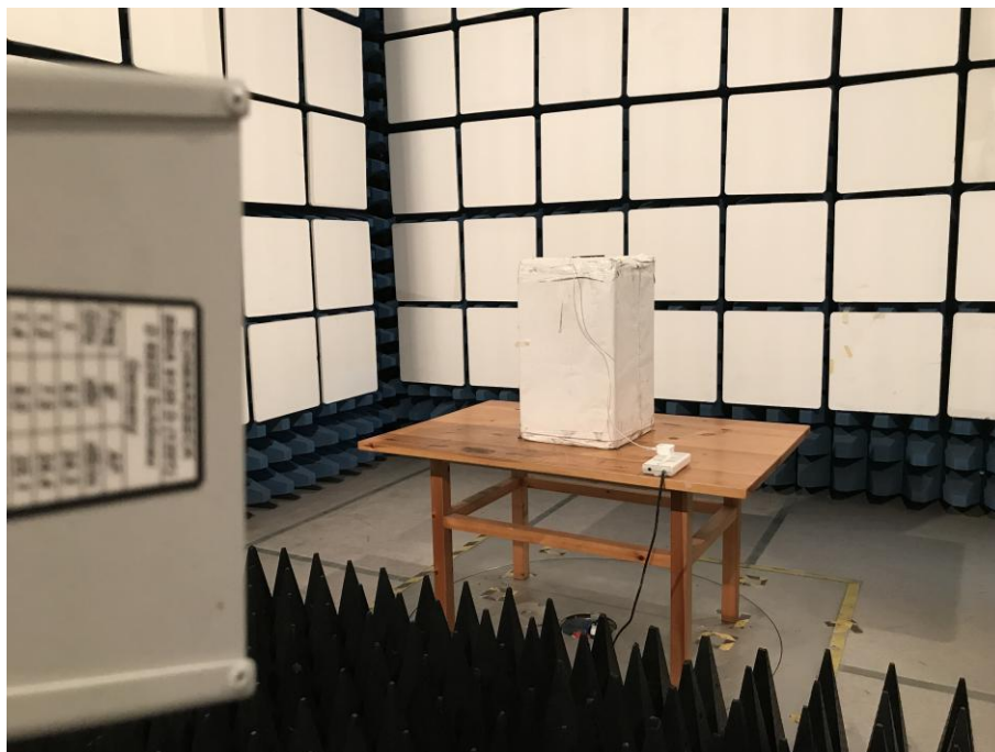
Above 1GHz-WIFI
