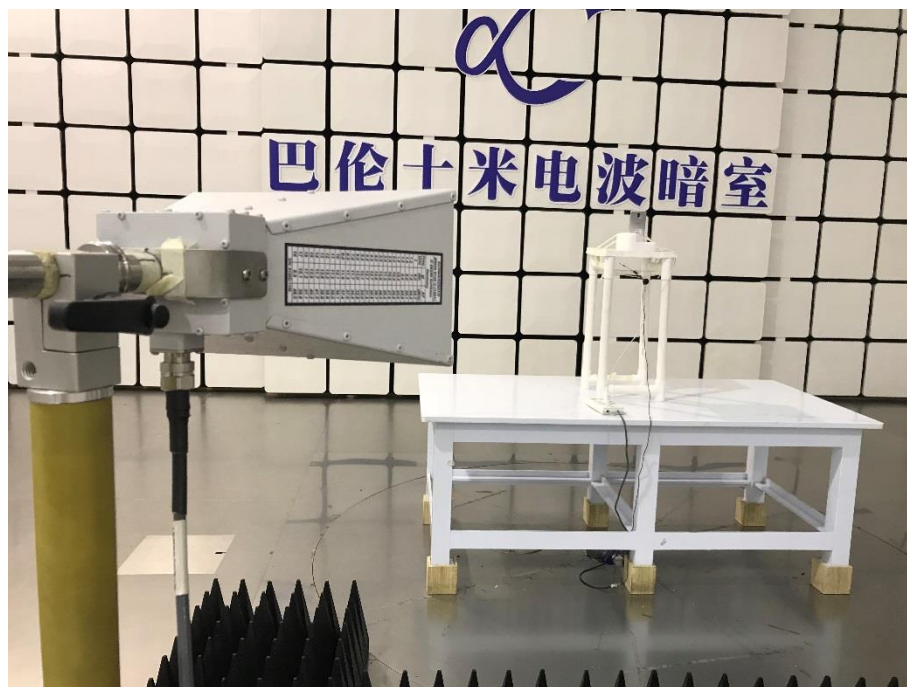
Above 1GHz-BT/BLE
