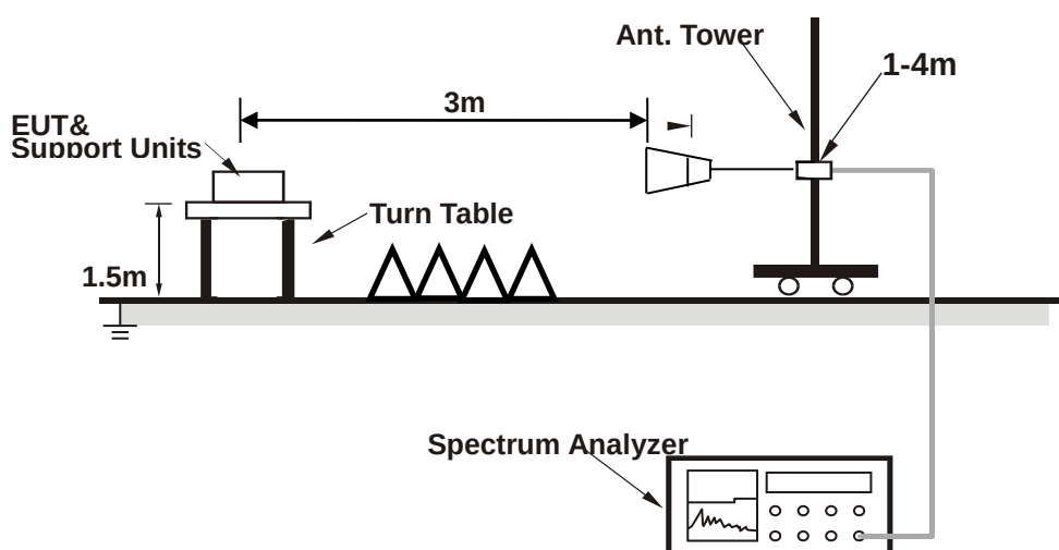
Setup diagram for Radiation (Above1G) Test
