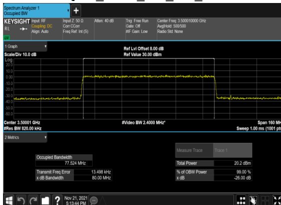
B5_N77(80M)_CP-OFDM_256 QAM_Outer_Full_Mid_CH
