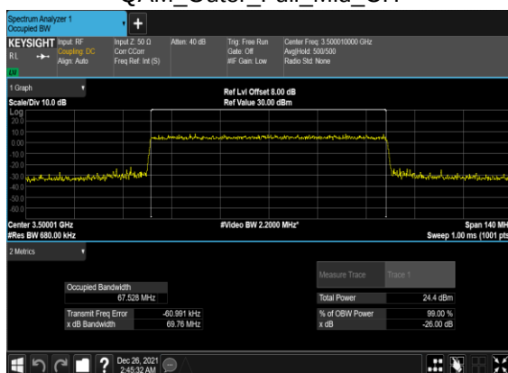
B5_N77(70M)_CP-OFDM_64 QAM_Outer_Full_Mid_CH
