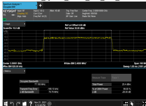
B5_N77(80M)_DFT-s- OFDM_QPSK_Outer_Full_Mid_CH
