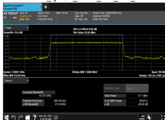
B5_N77(50M)_DFT-s- OFDM_QPSK_Outer_Full_Mid_CH
