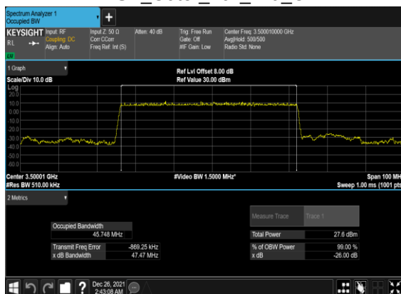
B5_N77(50M)_DFT-s-OFDM_PI_2- BPSK_Outer_Full_Mid_CH
