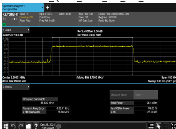
B5_N77(90M)_DFT-s- OFDM_QPSK_Outer_Full_Mid_CH
