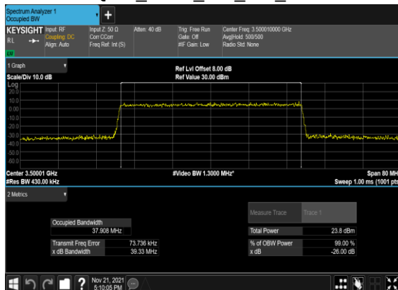
B5_N77(40M)_CP-OFDM_64 QAM_Outer_Full_Mid_CH
