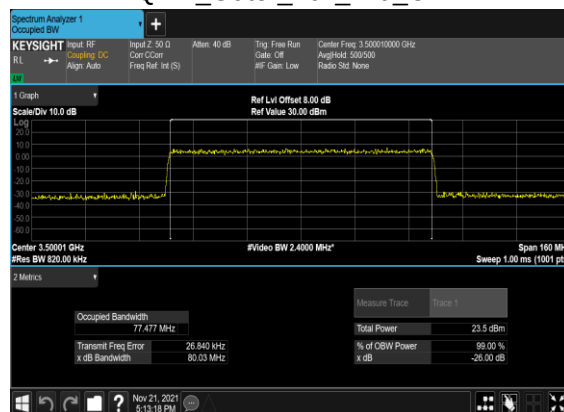
B5_N77(80M)_CP-OFDM_16 QAM_Outer_Full_Mid_CH
