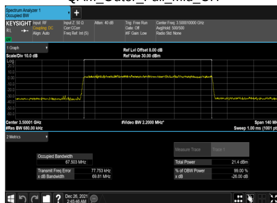
B5_N77(70M)_CP-OFDM_256 QAM_Outer_Full_Mid_CH
