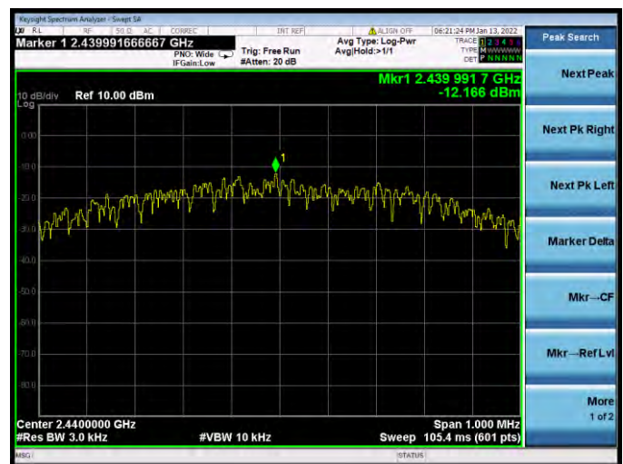
GFSK (BLE) MIDDLE CHANNEL
