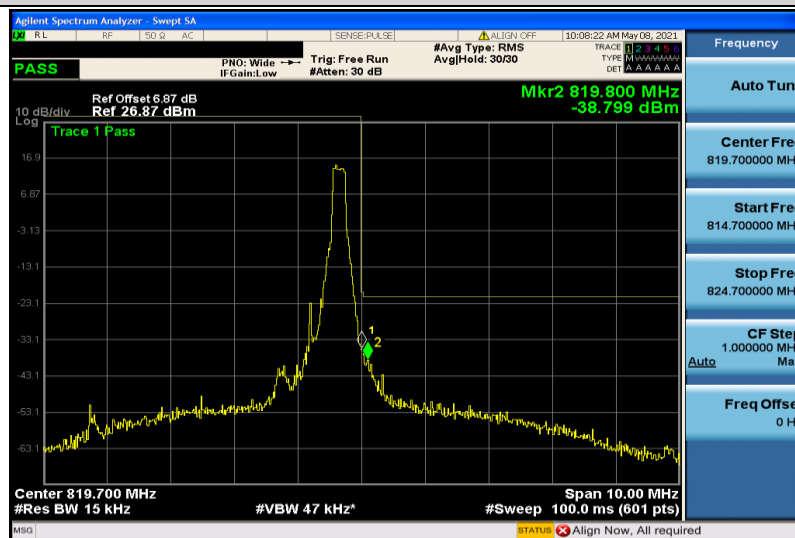
Band26-1.4MHz-16QAM-26740-1RB#5
