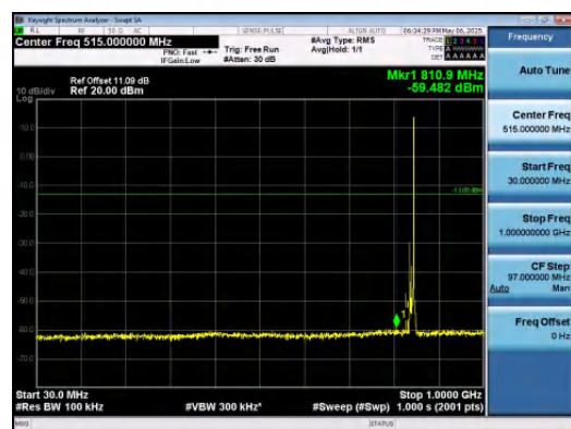
Band5-10MHz-QPSK-20600-1RB#49-30~1000-P ASS
