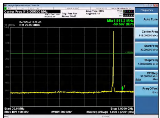
Band5-10MHz-QPSK-20525-1RB#49-30~1000-P ASS
