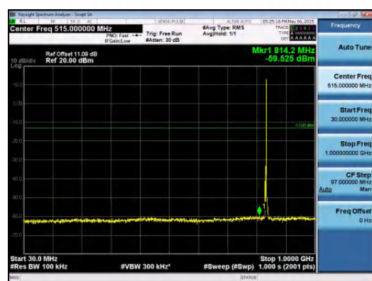
Band5-3MHz-QPSK-20525-1RB#14-30~1000-P
