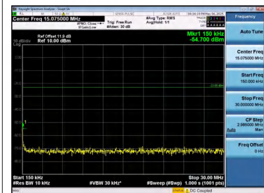
Band5-10MHz-QPSK-20600-1RB#49-0.15~30-P ASS
