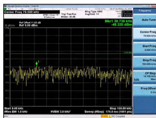
Band5-5MHz-QPSK-20525-1RB#24-0.009~0.15- PASS
