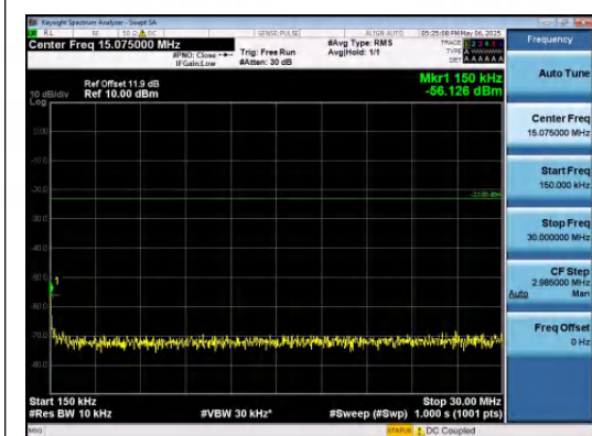
Band5-3MHz-QPSK-20525-1RB#14-0.15~30-PA
