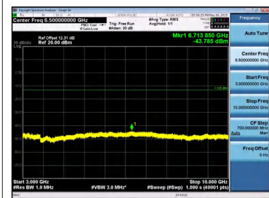
Band5-5MHz-QPSK-20525-1RB#0-3000~10000- PASS
