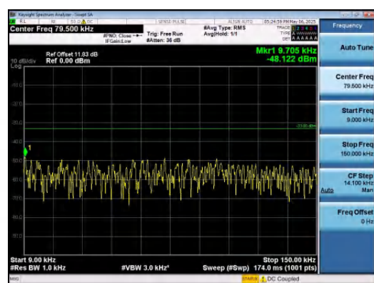
Band5-3MHz-QPSK-20525-1RB#14-0.009~0.15-
