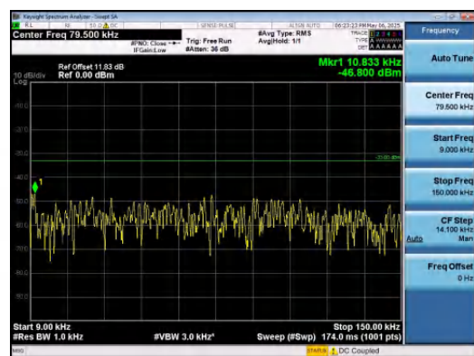
Band5-10MHz-QPSK-20450-1RB#49-0.009~0.1 5-PASS
