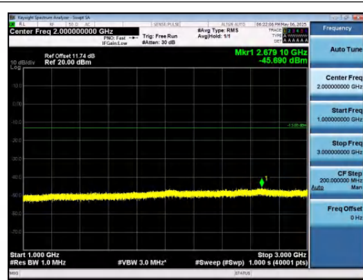
Band5-10MHz-QPSK-20450-1RB#0-1000~3000- PASS
