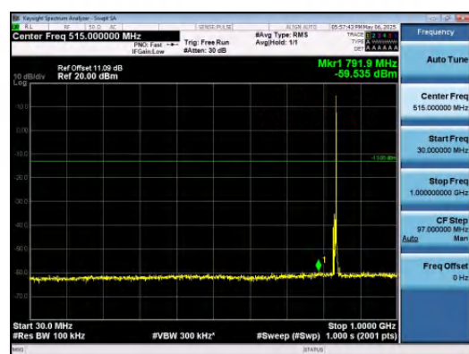
Band5-5MHz-QPSK-20525-1RB#24-30~1000-P ASS
