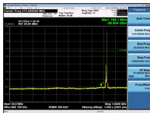
Band5-10MHz-QPSK-20450-1RB#49-30~1000-P ASS
