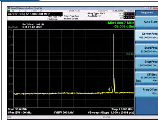
Band5-5MHz-QPSK-20525-1RB#0-30~1000-PA SS
