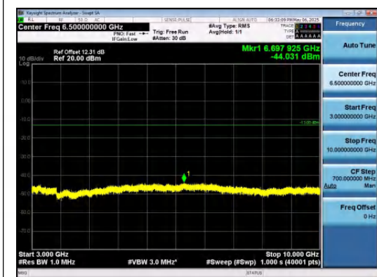
Band5-10MHz-QPSK-20600-1RB#0-3000~1000 0-PASS
