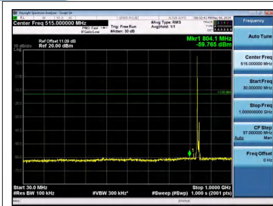
Band5-10MHz-QPSK-20600-1RB#0-30~1000-P ASS
