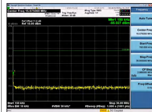
Band5-10MHz-QPSK-20525-1RB#49-0.15~30-P ASS
