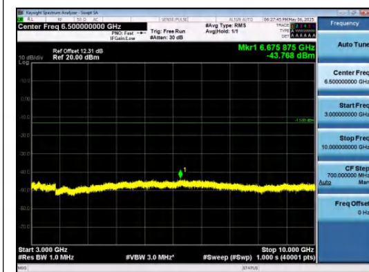
Band5-10MHz-QPSK-20525-1RB#0-3000~1000 0-PASS
