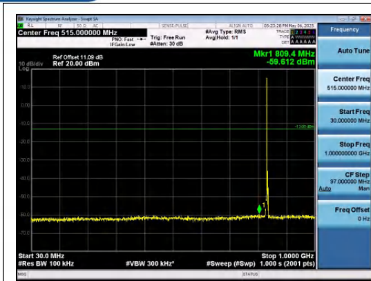
Band5-3MHz-QPSK-20525-1RB#0-30~1000-PA
