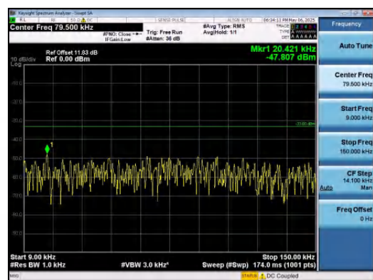
Band5-10MHz-QPSK-20600-1RB#49-0.009~0.1 5-PASS
