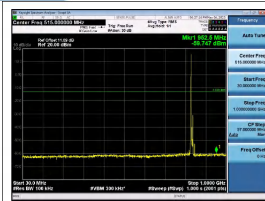
Band5-10MHz-QPSK-20525-1RB#0-30~1000-P ASS
