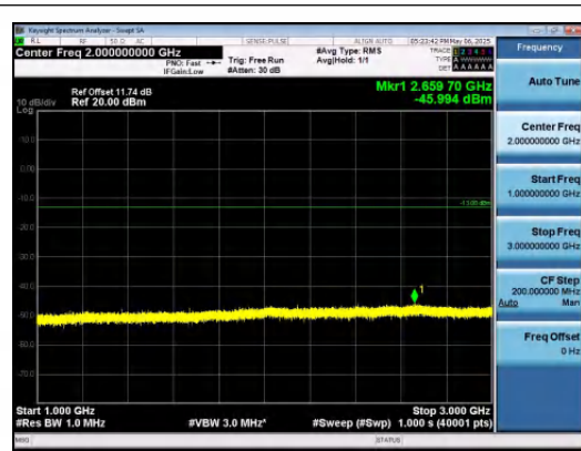
Band5-3MHz-QPSK-20525-1RB#0-1000~3000-P
