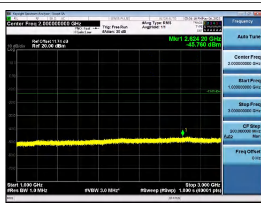
Band5-5MHz-QPSK-20525-1RB#0-1000~3000-P ASS
