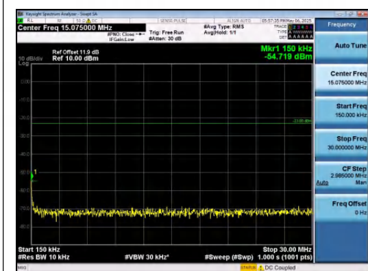
Band5-5MHz-QPSK-20525-1RB#24-0.15~30-PA SS
