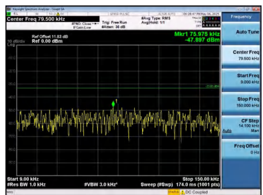
Band5-10MHz-QPSK-20525-1RB#49-0.009~0.1 5-PASS
