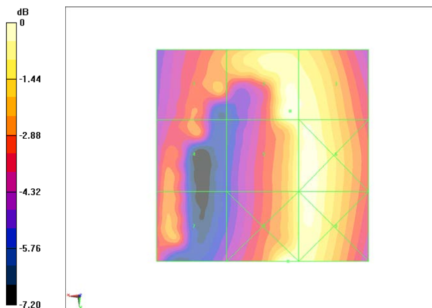
Fig B.9 HAC RF E-Field CDMA 835 Low
