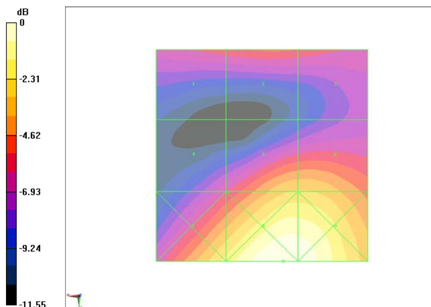
Fig B.10 HAC RF E-Field CDMA 1900 High
