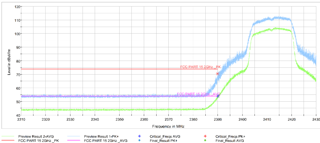
Fig.A.6.2.3 Transmitter Spurious Emission - Radiated (Power): 802.11g, ch1, 2.31 GHz - 2.43GHz
