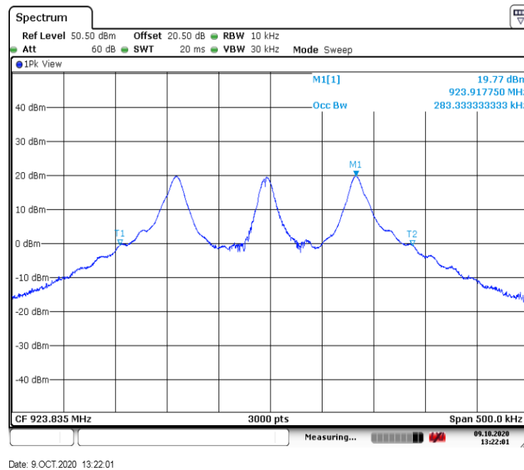
Figure 8.4-6: 99% Occupied bandwidth on high channel
