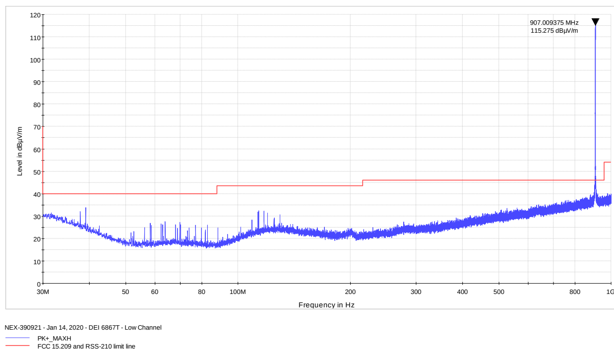
Figure 8.6-8: Radiated spurious (out-of-band) emissions, below 1 GHz low channel
