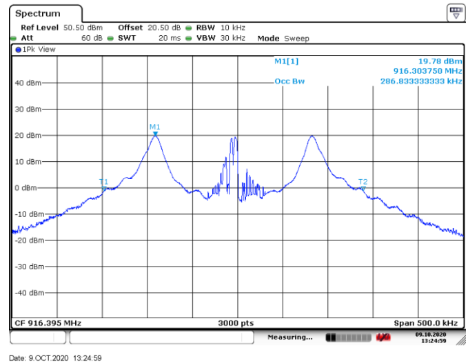
Figure 8.4-5: 99% Occupied bandwidth on mid channel
