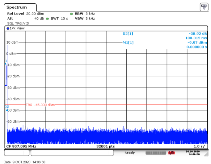
Figure 8.4-10: Dwell time, 10 s
