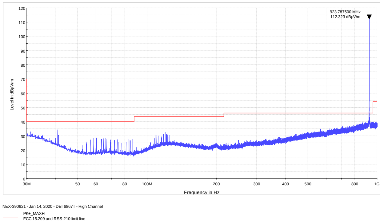
Figure 8.6-10: Radiated spurious (out-of-band) emissions, below 1 GHz high channel
