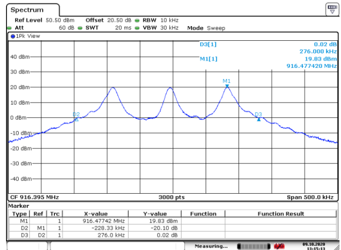
Figure 8.4-2: 20 dB bandwidth on mid channel
