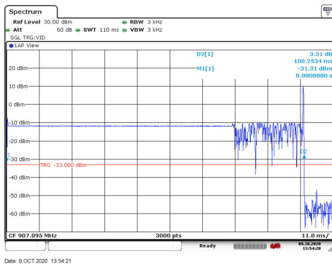
Figure 8.4-9: Dwell time, 100 ms
