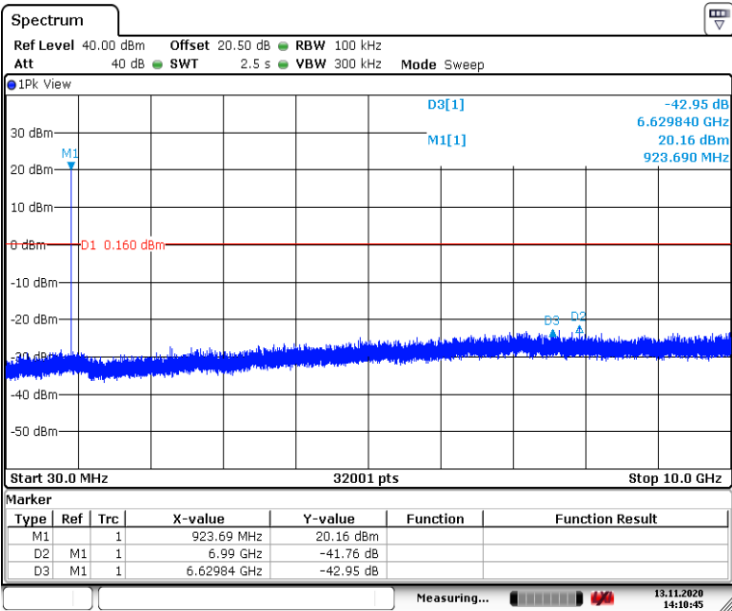
Figure 8.6-7: Conducted spurious emission, high channel
