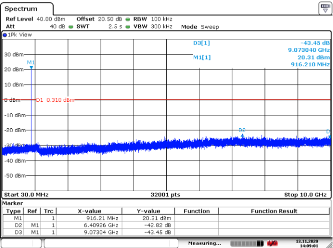
Figure 8.6-6: Conducted spurious emission, mid channel
