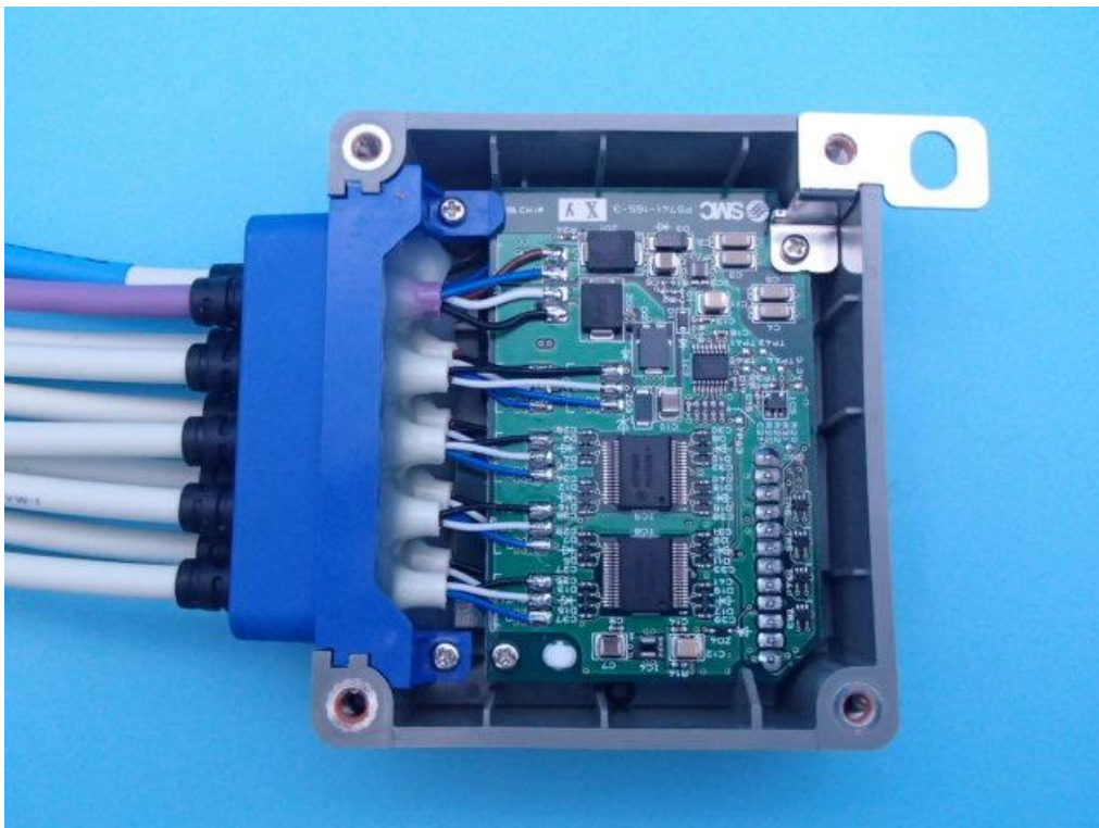
EX600-WDYA1 Inside view
