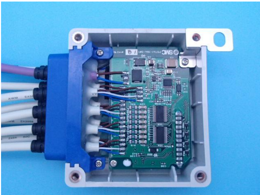
EX600-WDXA1 InSide view
